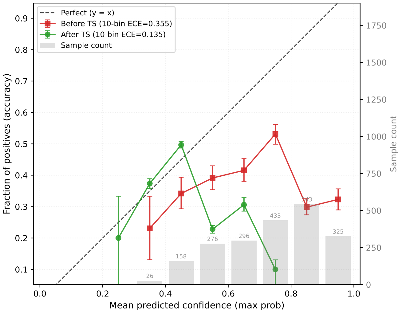
PTBXL \rightarrow CPSC (resnet1d, seed43) OOD target-test (n=2057, T=2.515)
