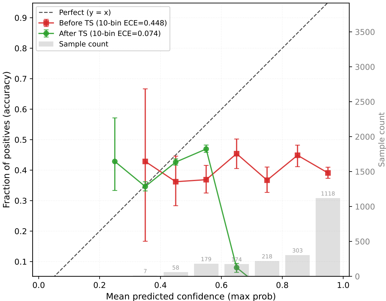
PTBXL \rightarrow CPSC (resnet1d, seed44) OOD target-test (n=2057, T=4.440)
