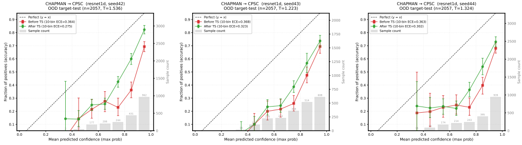
Figure 10: Chapman \rightarrow CPSC reliability diagrams: ResNet1D seeds 42–44.
