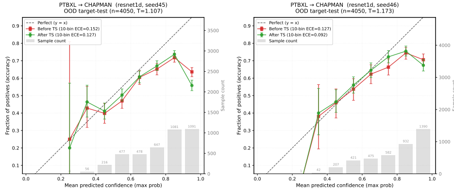
Figure 27: PTB-XL→Chapman reliability diagrams: ResNet1D seeds 45–46.
