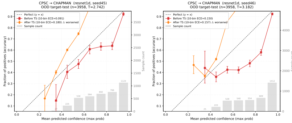
Figure 19: CPSC→Chapman reliability diagrams: ResNet1D seeds 45–46.
