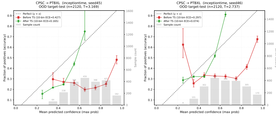
Figure 25: CPSC→PTB-XL reliability diagrams: InceptionTime seeds 45–46.
