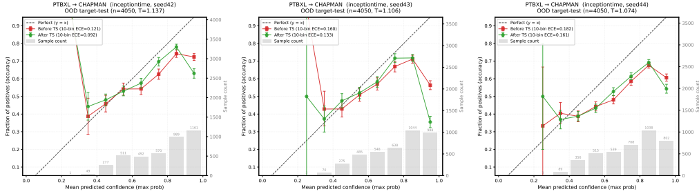
Figure 28: PTB-XL→Chapman reliability diagrams: InceptionTime seeds 42–44.
