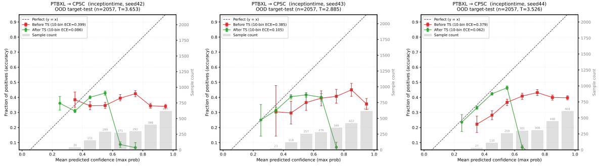
Figure 23: PTB-XL→CPSC reliability diagrams: InceptionTime seeds 42–44.
