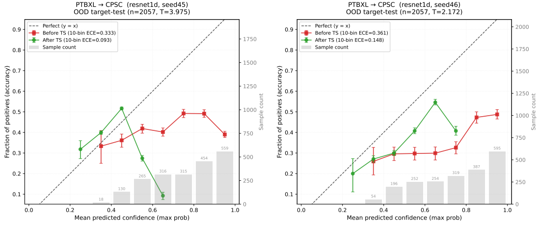
Figure 22: PTB-XL→CPSC reliability diagrams: ResNet1D seeds 45–46.
