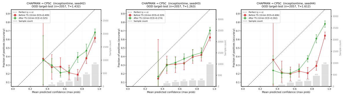
Figure 3: Chapman→CPSC reliability diagrams: InceptionTime seeds 42–44.
