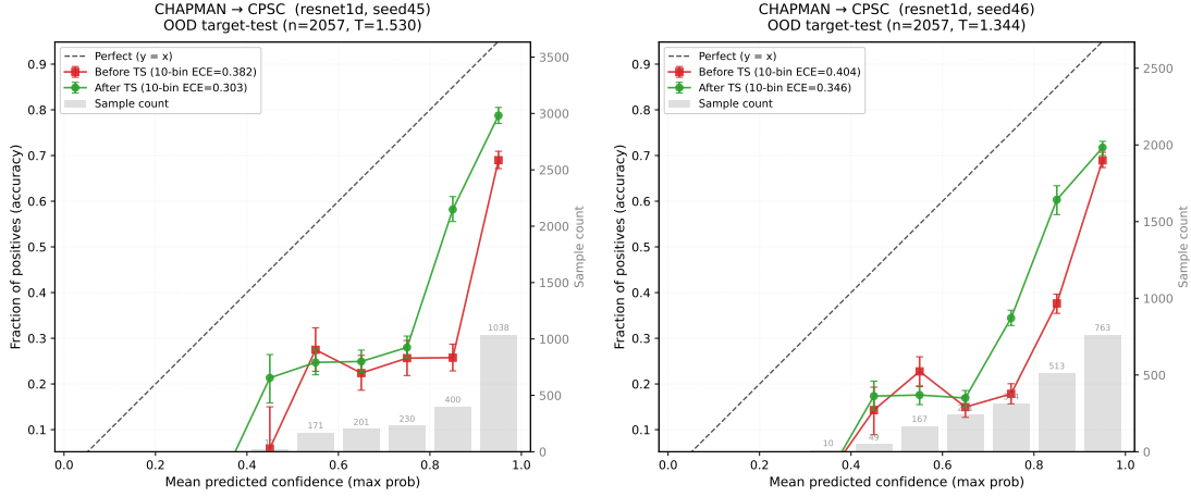
Figure 2: Chapman→CPSC reliability diagrams: ResNet1D seeds 45–46.
