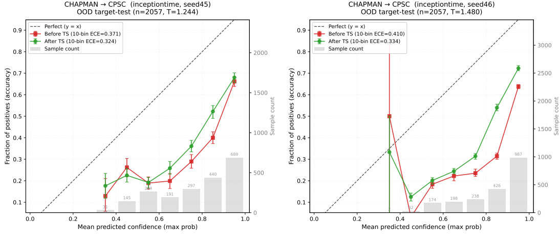
Figure 4: Chapman→CPSC reliability diagrams: InceptionTime seeds 45–46.
