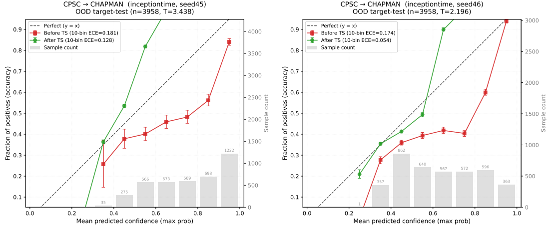
Figure 12: CPSC→Chapman reliability diagrams: InceptionTime seeds 45–46.
