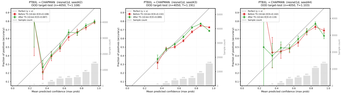
Figure 17: PTB-XL→Chapman reliability diagrams: ResNet1D seeds 42–44.
