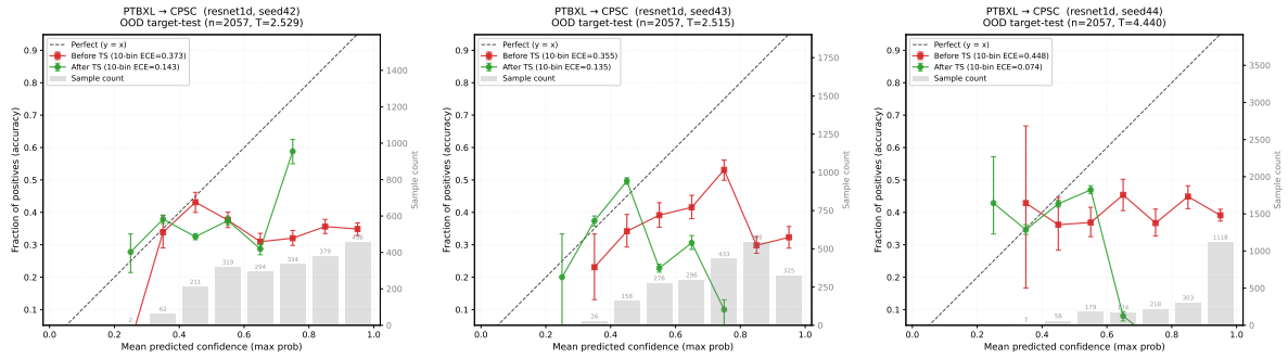
Figure 21: PTB-XL→CPSC reliability diagrams: ResNet1D seeds 42–44.
