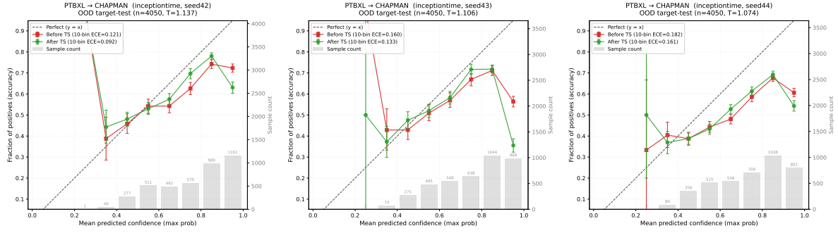
Figure 19: PTB-XL→Chapman reliability diagrams: InceptionTime seeds 42–44.
