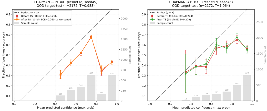
Figure 6: Chapman→PTB-XL reliability diagrams: ResNet1D seeds 45–46.
