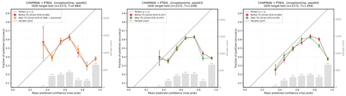
Figure 7: Chapman→PTB-XL reliability diagrams: InceptionTime seeds 42–44.
