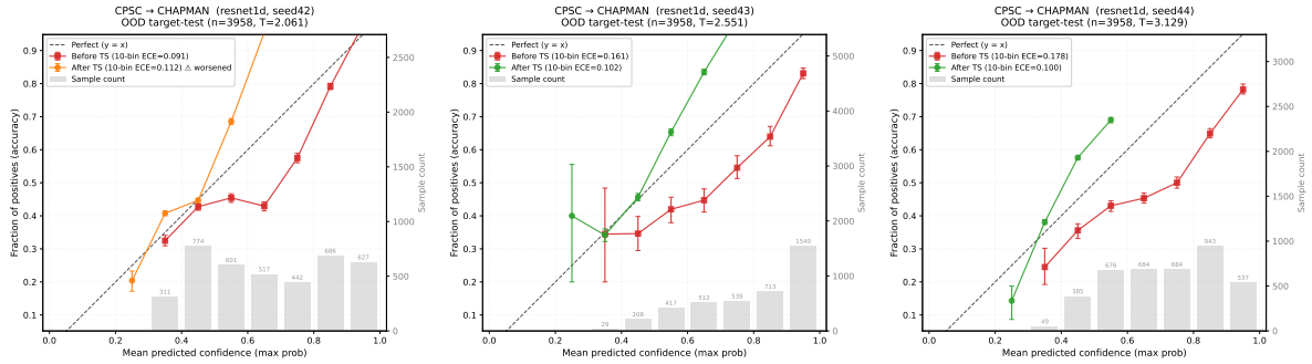
Figure 9: CPSC→Chapman reliability diagrams: ResNet1D seeds 42–44.
