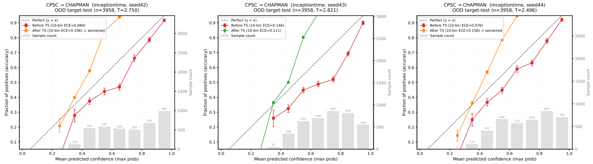
Figure 11: CPSC→Chapman reliability diagrams: InceptionTime seeds 42–44.
