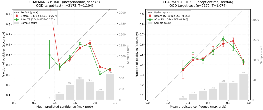
Figure 8: Chapman→PTB-XL reliability diagrams: InceptionTime seeds 45–46.
