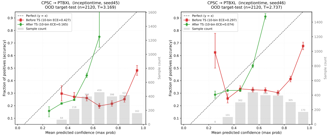
Figure 16: CPSC→PTB-XL reliability diagrams: InceptionTime seeds 45–46.
