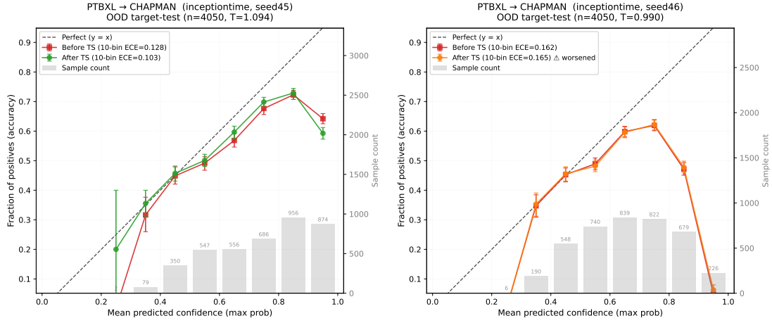
Figure 20: PTB-XL→Chapman reliability diagrams: InceptionTime seeds 45–46.
