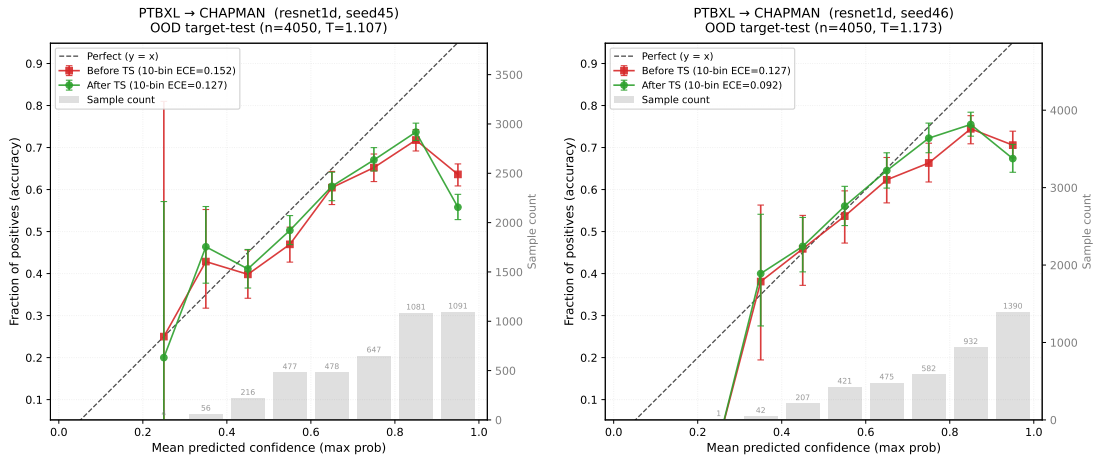
Figure 18: PTB-XL→Chapman reliability diagrams: ResNet1D seeds 45–46.
