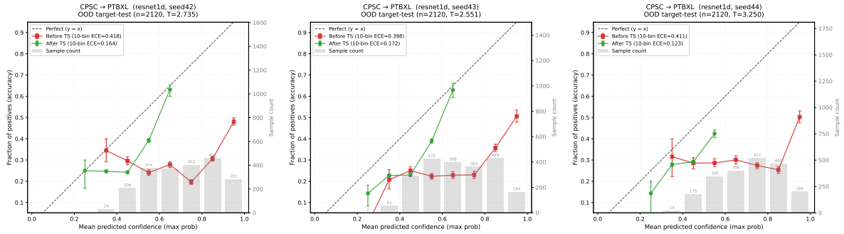
Figure 13: CPSC→PTB-XL reliability diagrams: ResNet1D seeds 42–44.
