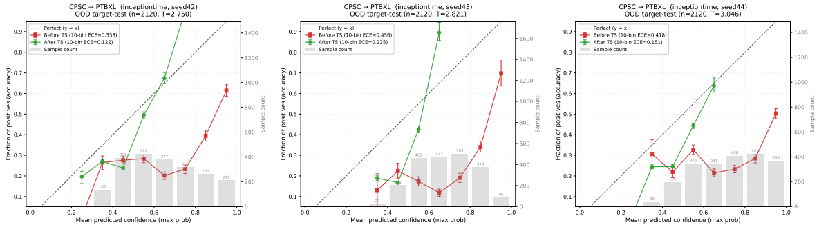
Figure 15: CPSC→PTB-XL reliability diagrams: InceptionTime seeds 42–44.
