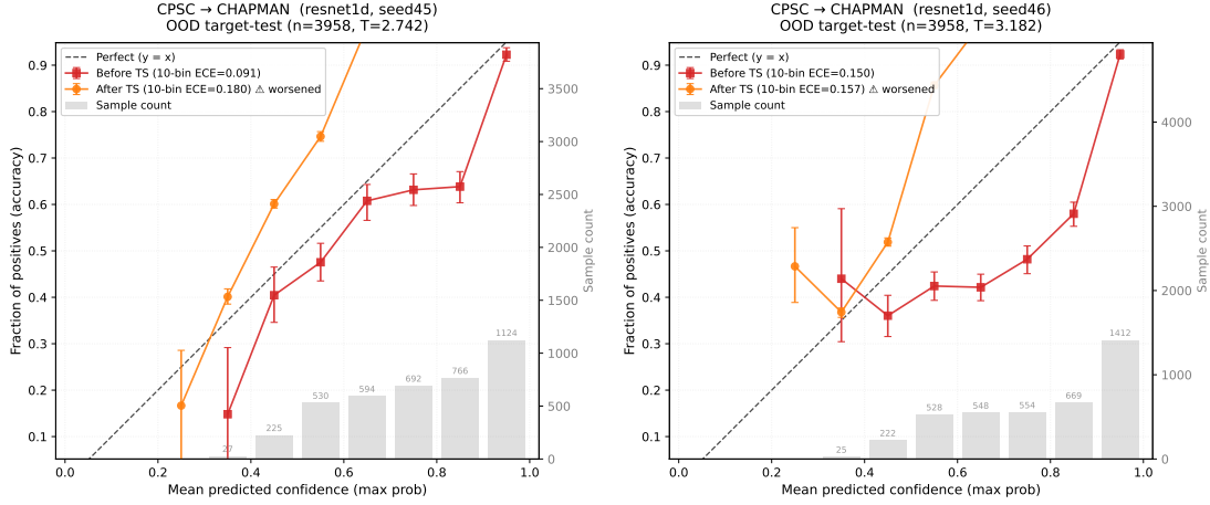
Figure 10: CPSC→Chapman reliability diagrams: ResNet1D seeds 45–46.
