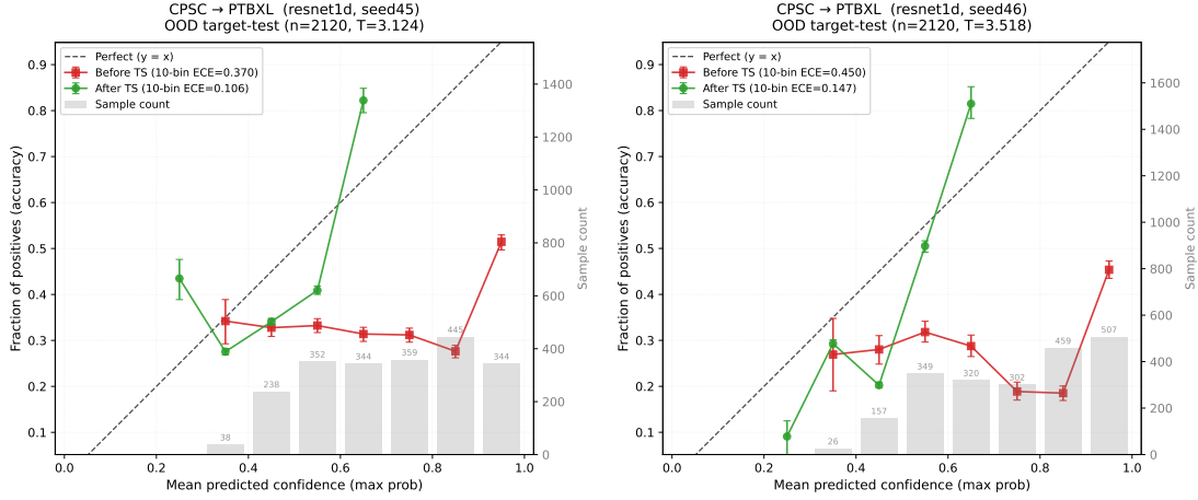
Figure 14: CPSC→PTB-XL reliability diagrams: ResNet1D seeds 45–46.
