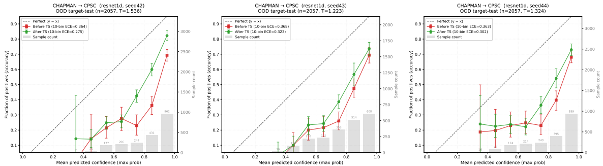
Figure 1: Chapman \rightarrow CPSC reliability diagrams: ResNet1D seeds 42–44.
