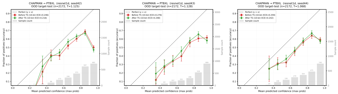
Figure 5: Chapman→PTB-XL reliability diagrams: ResNet1D seeds 42–44.
