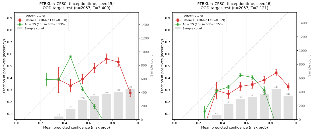
Figure 24: PTB-XL→CPSC reliability diagrams: InceptionTime seeds 45–46.
