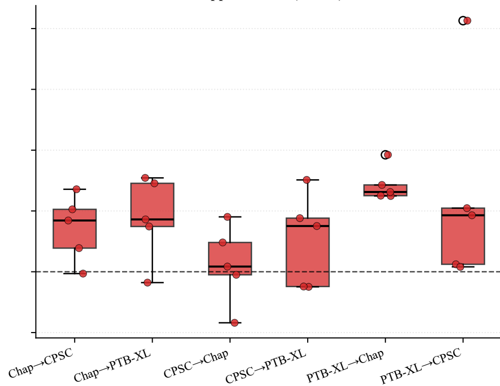
ResNet1D Support: 24/30 (80.0%)
