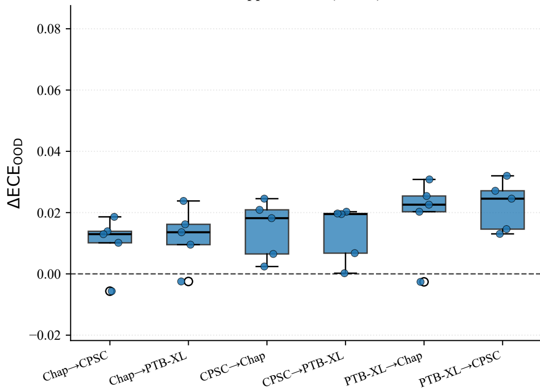
InceptionTime Support: 27/30 (90.0%)
