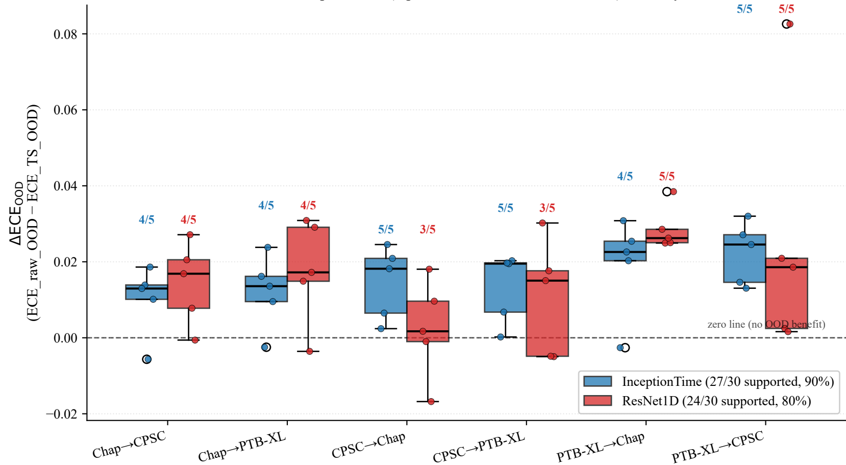
Primary Endpoint: OOD Calibration Benefit by Transfer Direction 60 seed experiments (6 pairs \times 2 architectures \times 5 seeds), TS only
