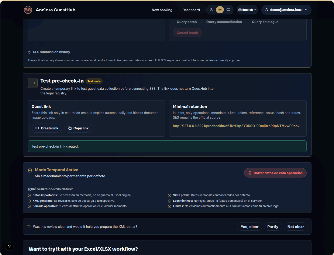
SES and test pre-check-in panel
