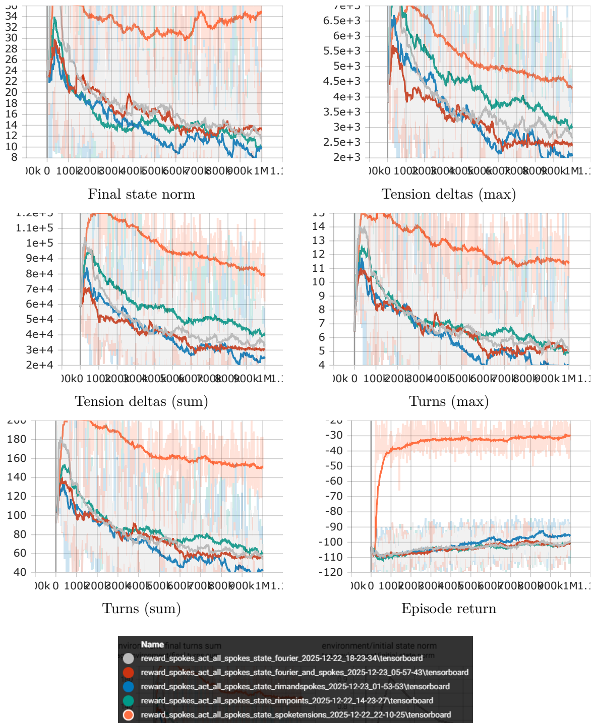
Overview of TD-MPC training metrics (spokes_all_spokes).
