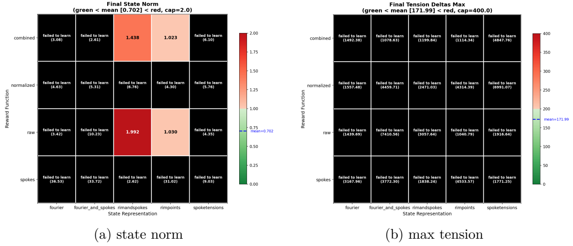
Figure 4.4: PPO continuous
