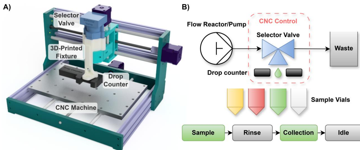
Figure 1. Schematic and hardware overview of the solvent-resistant, Python-controlled fraction collector. A) CAD rendering of the system, built on a 3-axis CNC platform for automated vial positioning, with a drop counter for real-time volume monitoring and a 3D-printed fixture securing the selector valve. B) Functional flow diagram showing integration with upstream flow reactors or pumps. A selector valve alternates between sample collection and waste modes. Droplet formation is monitored by the drop counter, enabling accurate, volume-based fraction collection into user-defined sample vials. The bottom sequence illustrates the programmable collection cycle used to prevent cross-contamination.
