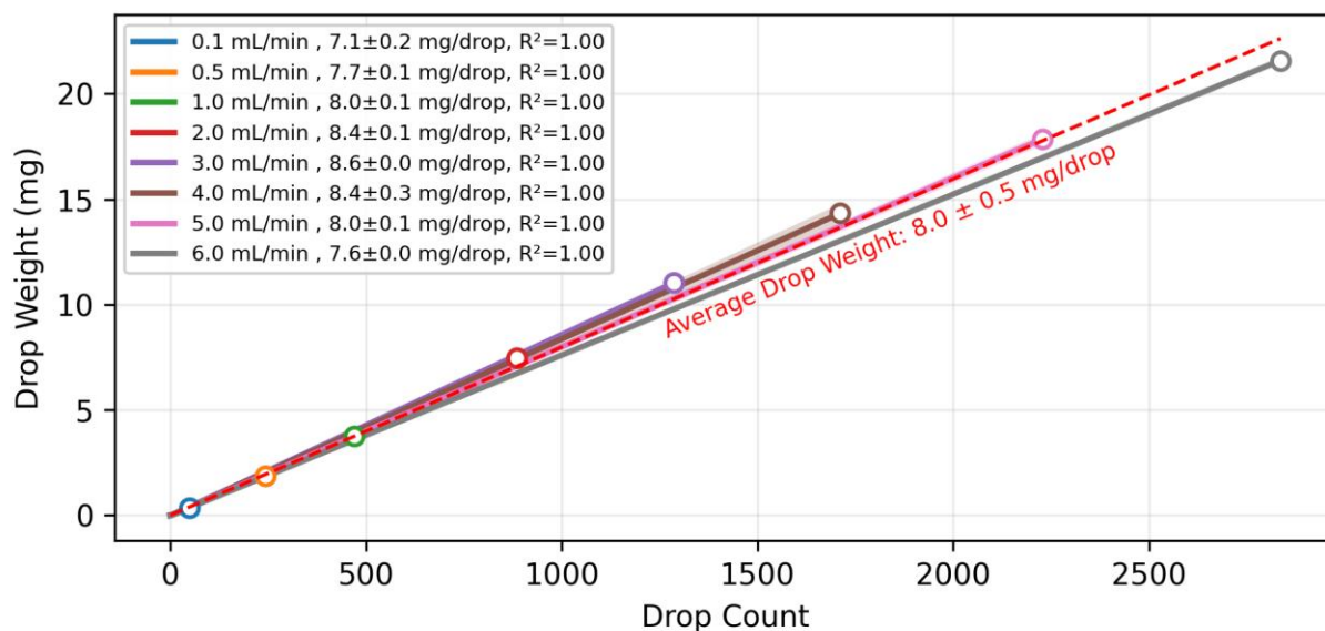
Figure 2. Collection accuracy tests of the fraction collector at different flow rates using IPA. The plot shows the relationship between the number of drops recorded by the drop counter and the corresponding collected weight at flow rates ranging from 0.1 to 6.0 mL/min. Each curve represents a different flow rate, with the associated droplet weight and linear fit ( R^2 ) summarised in the legend. Shaded regions represent the standard deviation across replicates for each flow rate. The average drop weight across the range of flow rates is shown as the red dashed line and the annotation.
