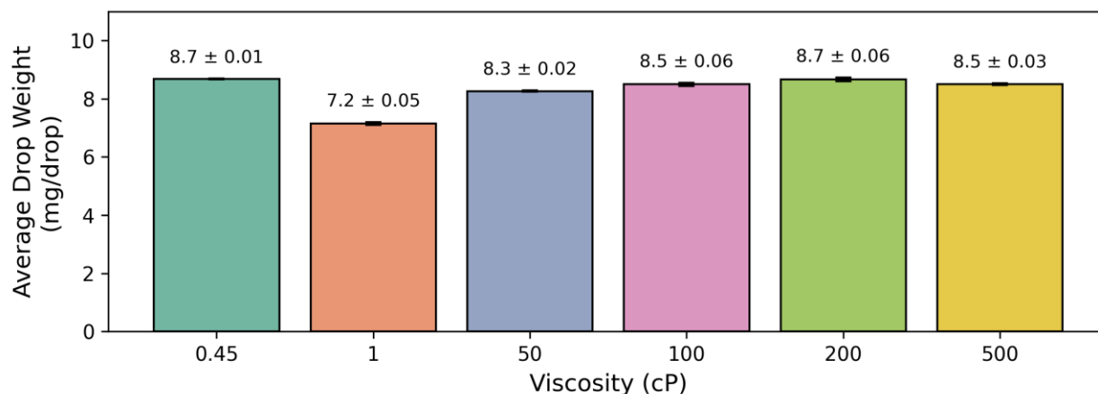
Figure 3. Average droplet weight measured by the drop-counter-based fraction collector at different fluid viscosities. Each bar represents the mean droplet weight obtained from three repeated tests using Siltech viscosity standards ranging from 1 to 500 cP and ethyl acetate (0.45 cP). Error bars indicate the standard deviation of droplet weight for each viscosity condition. The error bars represent the standard deviation calculated from three independent experiments.
