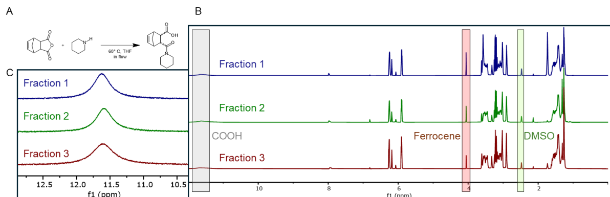
Figure 5. (A) Reaction scheme showing ring-opening of nadic anhydride with piperidine to form the amide-carboxylic acid product. (B) Overlay of 1 H NMR spectra (normalised to ferrocene internal standard) for three consecutive fractions collected at steady state. Key peaks highlighted: ferrocene (4.0 ppm, red box), DMSO-d 6 solvent (2.5 ppm, green box), and carboxylic acid proton (11.6 ppm, grey box). (C) Expanded view of the COOH region (10.5–12.5 ppm) showing excellent consistency across all three fractions (integrations: 5.51, 5.57 and 5.44 with reference to the ferrocene peak, set to 1.00)
