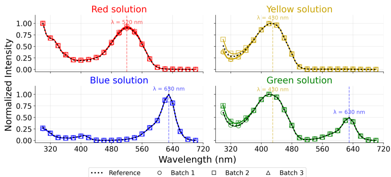
Figure 4. Absorbance spectra of food dye solutions collected by the fraction collector across three repeated batches. Each subplot shows the normalised absorbance intensity of the red, yellow, blue, and green dye solutions, measured using a plate reader. Dotted lines indicate reference spectra for each pure dye, while markers represent three independent collection batches. Characteristic absorption peaks of the colours are indicated as vertical dashed lines at \lambda = 520 nm (red), \lambda = 430 nm (yellow), and \lambda = 630 nm (blue).
