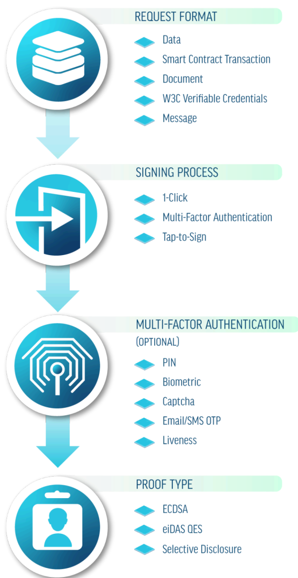
Figure 5: Digital Signature Process
