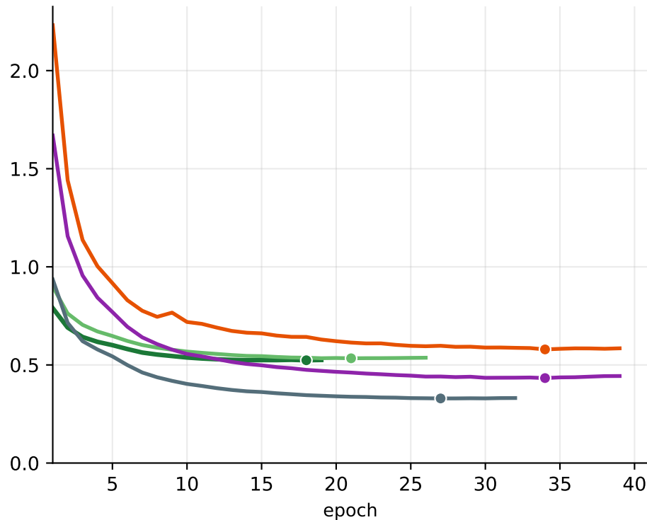
Stage-3 HAR-CoT
