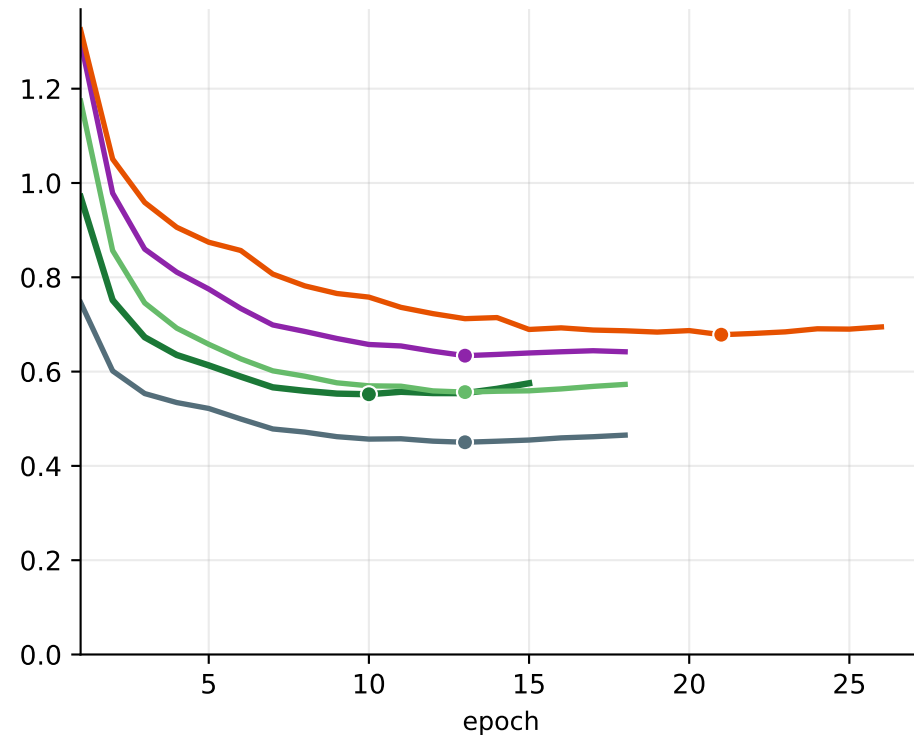
Stage-4 Sleep-CoT
