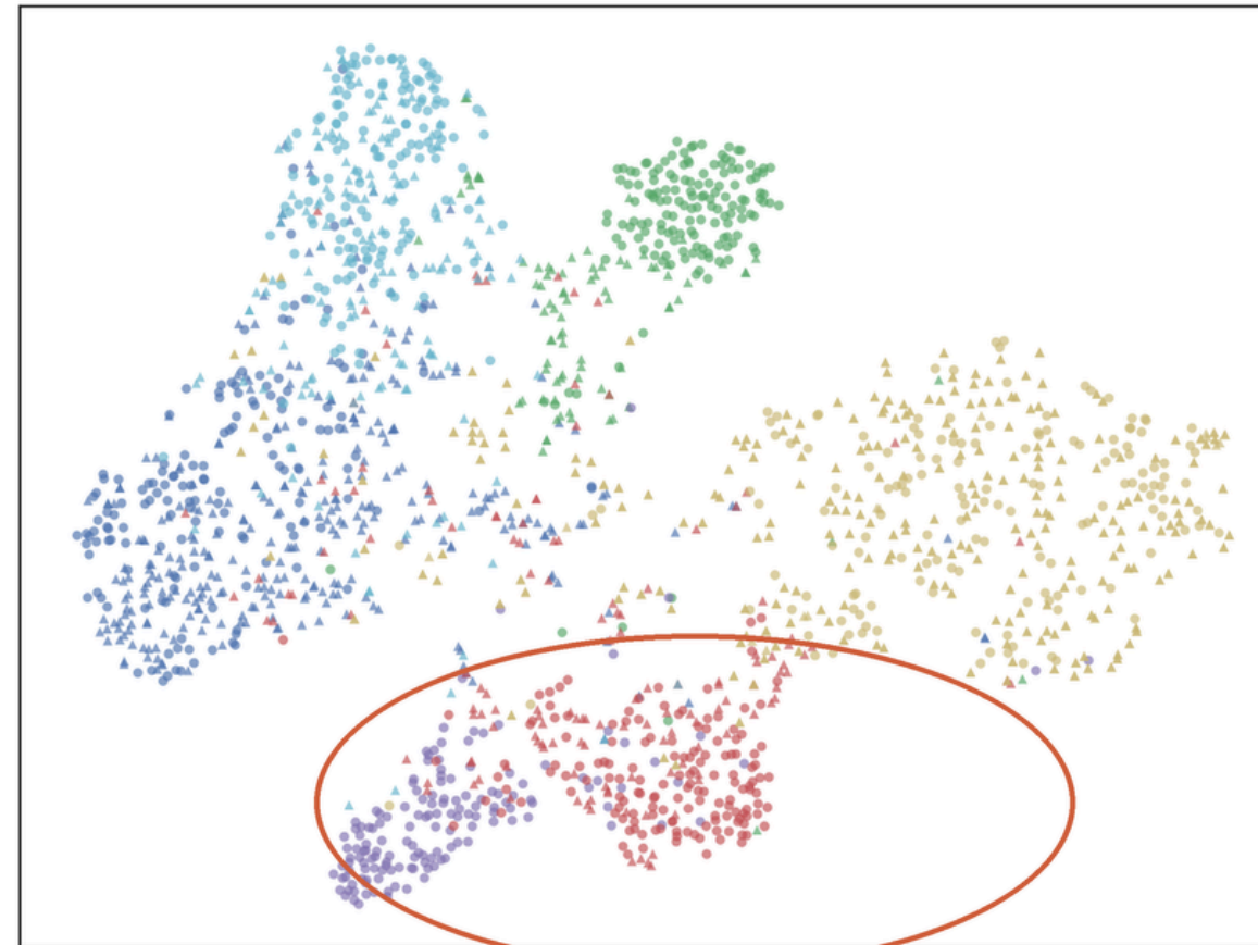
CORAL
