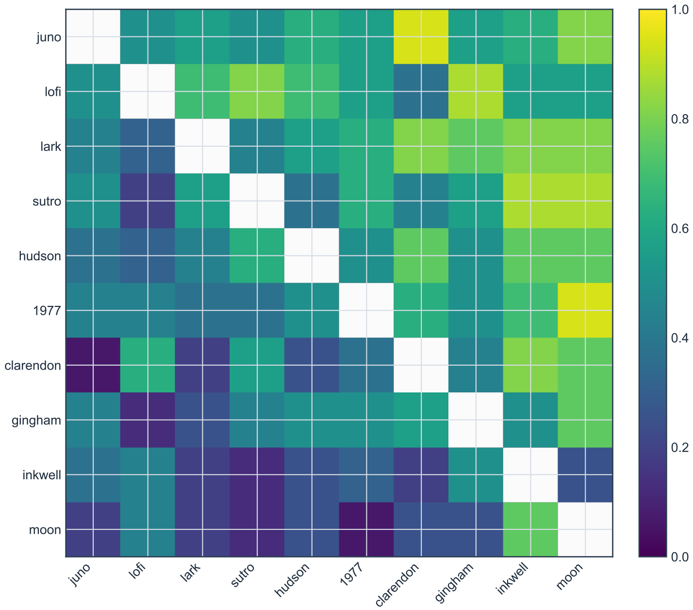
Ordered pairwise win-probability matrix (arousal)
