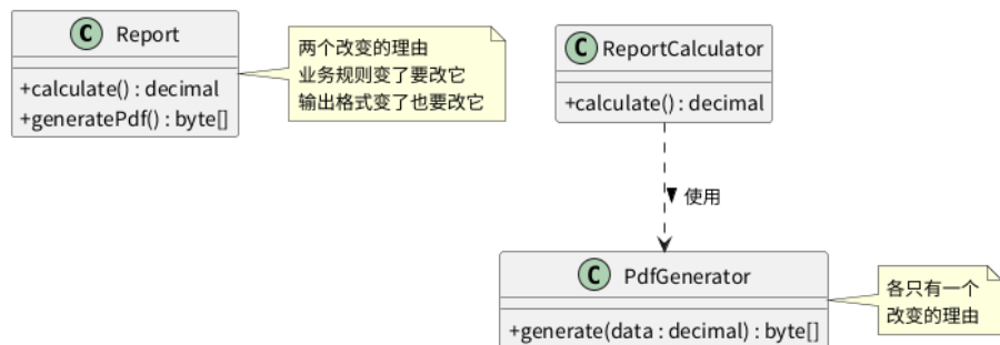
Figure 4: 单一职责
