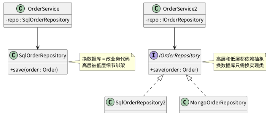
Figure 8: 依赖倒置
