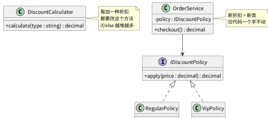
Figure 5: 开闭原则
