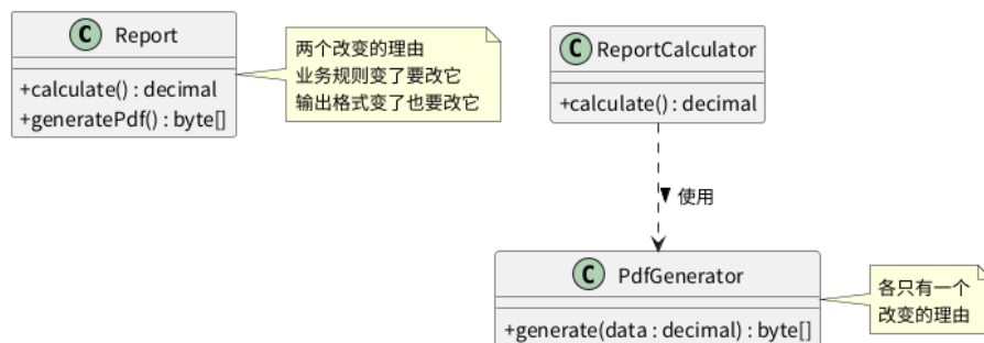
Figure 4: 单一职责
