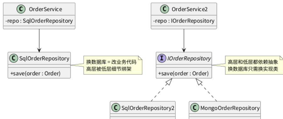
Figure 8: 依赖倒置
