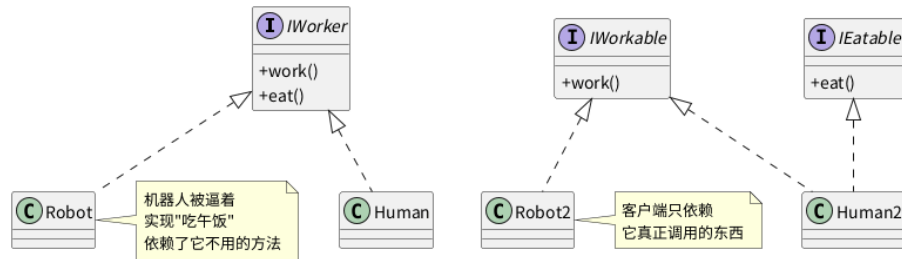
Figure 7: 接口隔离
