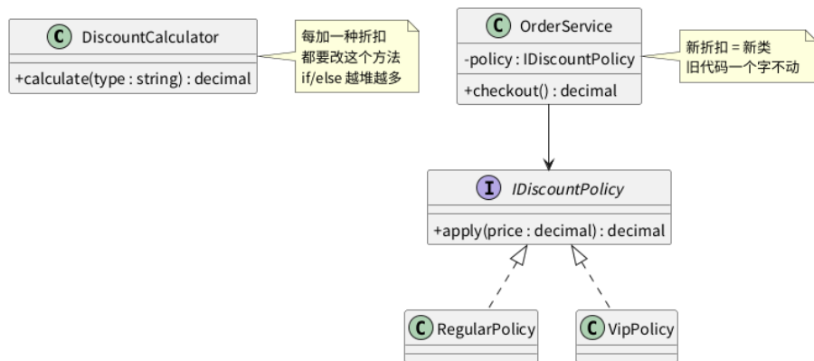
Figure 5: 开闭原则
