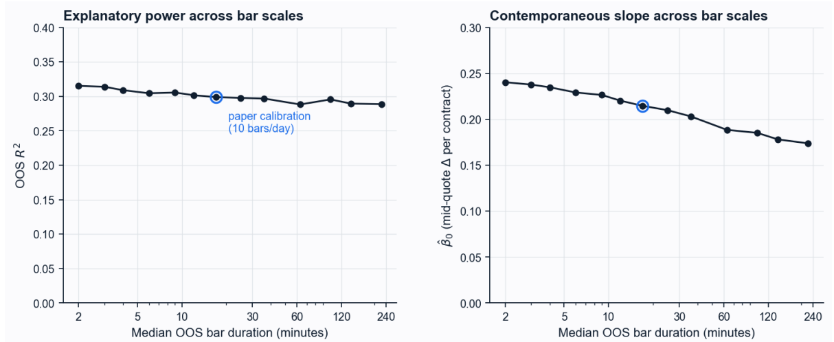
Figure 2: Out-of-sample R^2 (left) and contemporaneous slope \hat{\beta}_0 (right) as the bar threshold is varied from one to one hundred target bars per day, plotted against the resulting median OOS bar duration. The threshold is recalibrated on the in-sample window at each scale; the circled point is the ten-bars-per-day calibration used throughout the paper.
