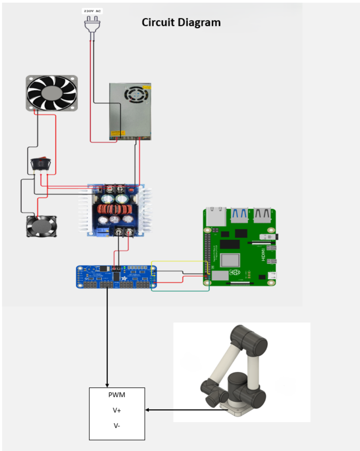
Figure 6: Detailed Circuit Diagram
