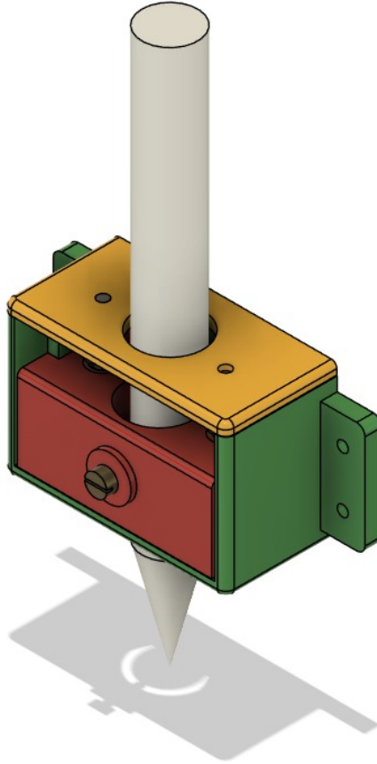
Figure 2: Schematic Diagram of the Pen Holder
