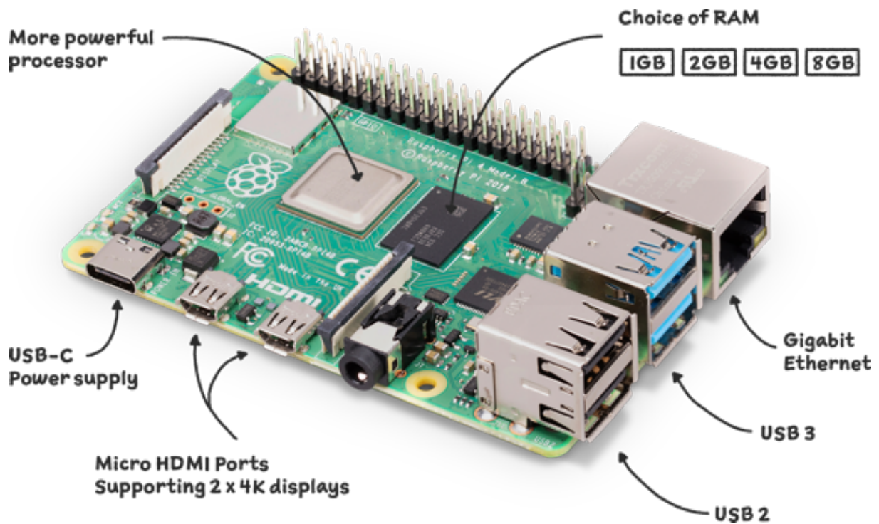
Figure 7: Raspberry Pi 4 Board
