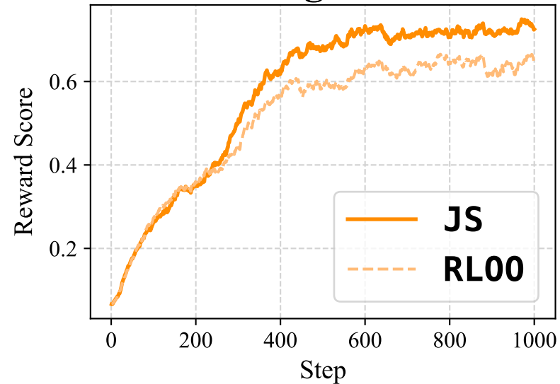
Training Reward
