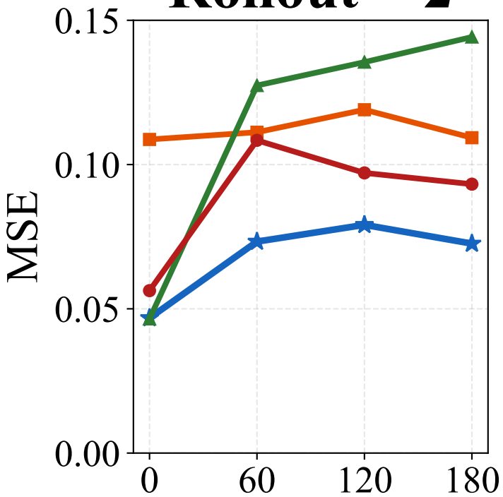
Rollout = 2
