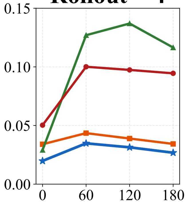
Rollout = 4
