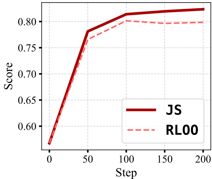
MATH500
