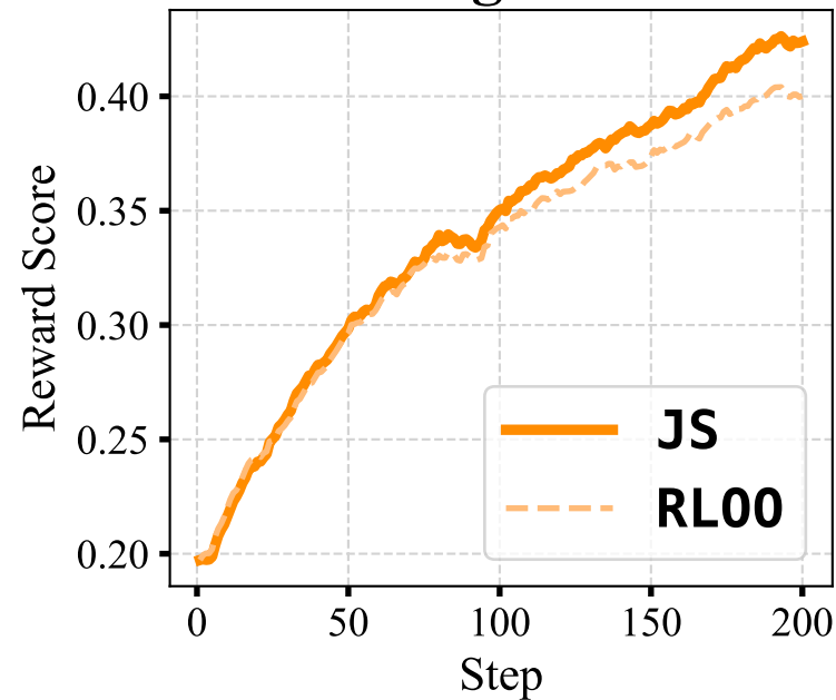
Training Reward
