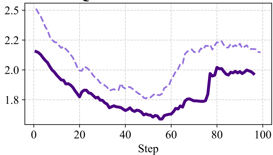
\times 10^{-6} Qwen2.5-Math-7B
