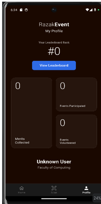
Figure 4: Profile Screen with Statistics and Leaderboard
