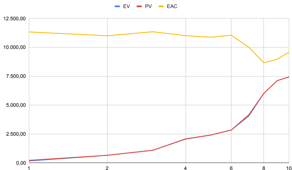
Figura 2: Planned Value - Earned Value
