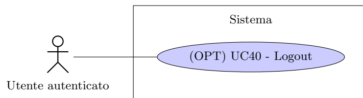
Figura 41: UC40 - Logout
