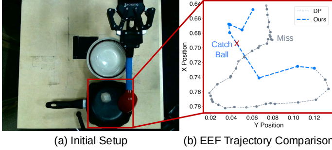
Fig. 6: Policy Execution Trajectory Comparison. (a) Initial setup for meatball scooping. (b) Comparison of end-effector (EEF) XY trajectories from our framework and a policy trained on robot-collected data. Our method generates smoother, more natural, and efficient trajectories with fewer waypoints, enabling fluid and precise motion. In contrast, the robot-collected policy produces jerky movements with excessive waypoints, which hinder task performance.
