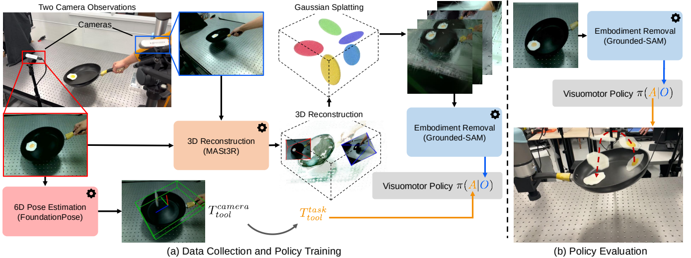
Fig. 2: Policy Design. Human play data was collected using two RGB cameras and processed through the foundation model MAST3R [34] to generate 3D reconstructions. Using 3D Gaussian splatting, we sampled novel views to augment the dataset. The human hand (embodiment) was segmented out from the images to create embodiment-agnostic observations, which serve as inputs to the policy. To label actions for policy training, a pose estimation model (FoundationPose [72] in this work) was used to extract the tool’s pose in the camera frame, T_{\text{tool}}^{\text{camera}} . A coordinate transformation was then applied to compute the tool’s pose in the task space, T_{\text{tool}}^{\text{task}} . Finally, a diffusion policy was implemented as the visuomotor policy to enable effective learning and execution.
