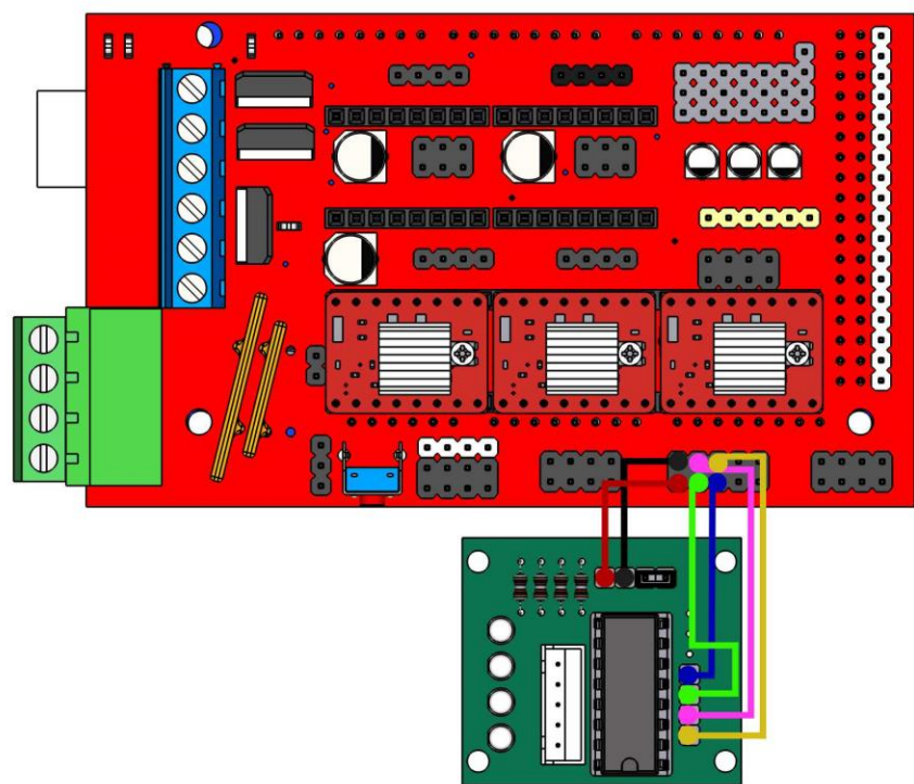
ULN2003 Stepper for driving 28BYJ-48 micro-stepper
