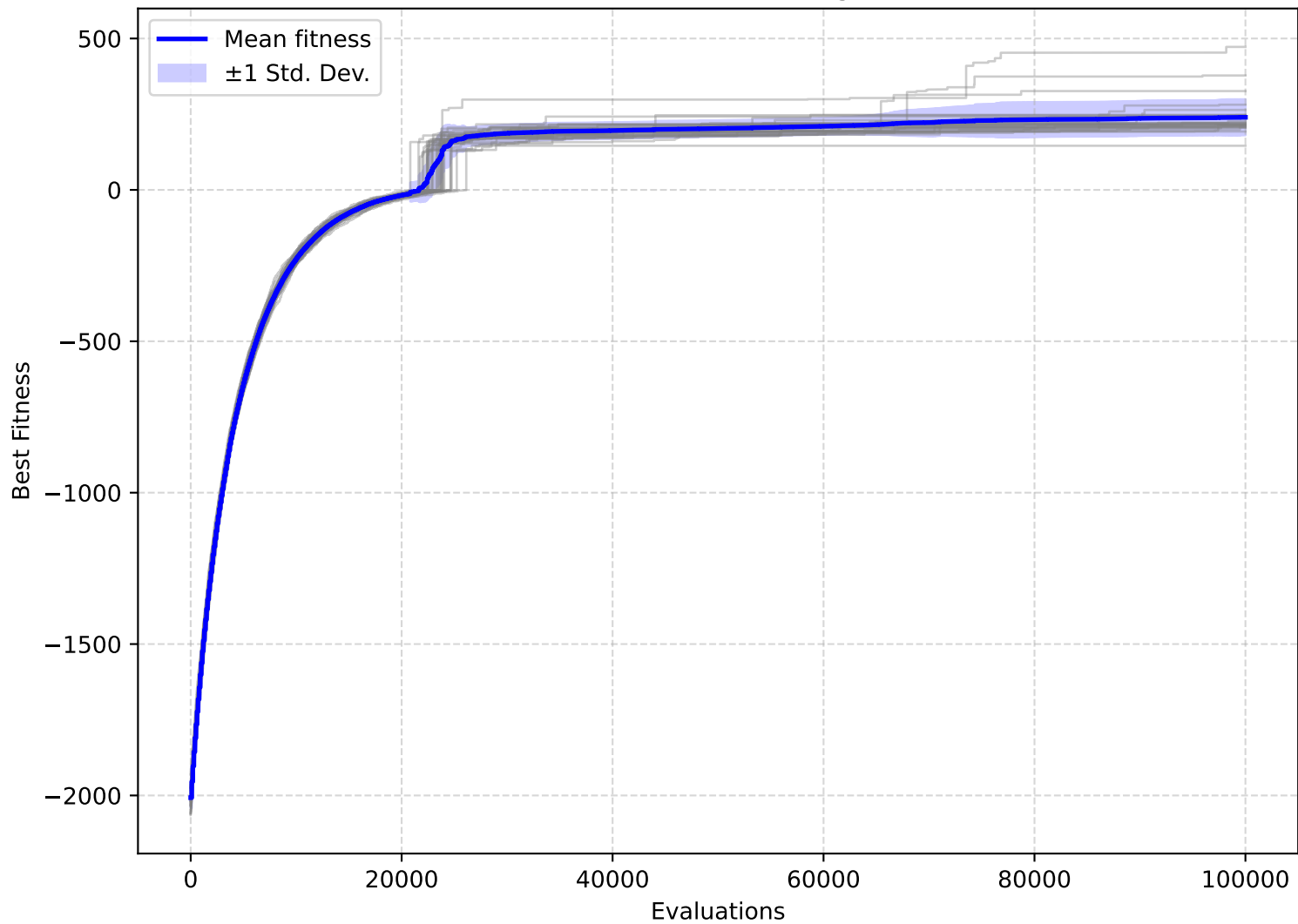
(1+1)EA/MaxInfluence — Convergence on F2201
