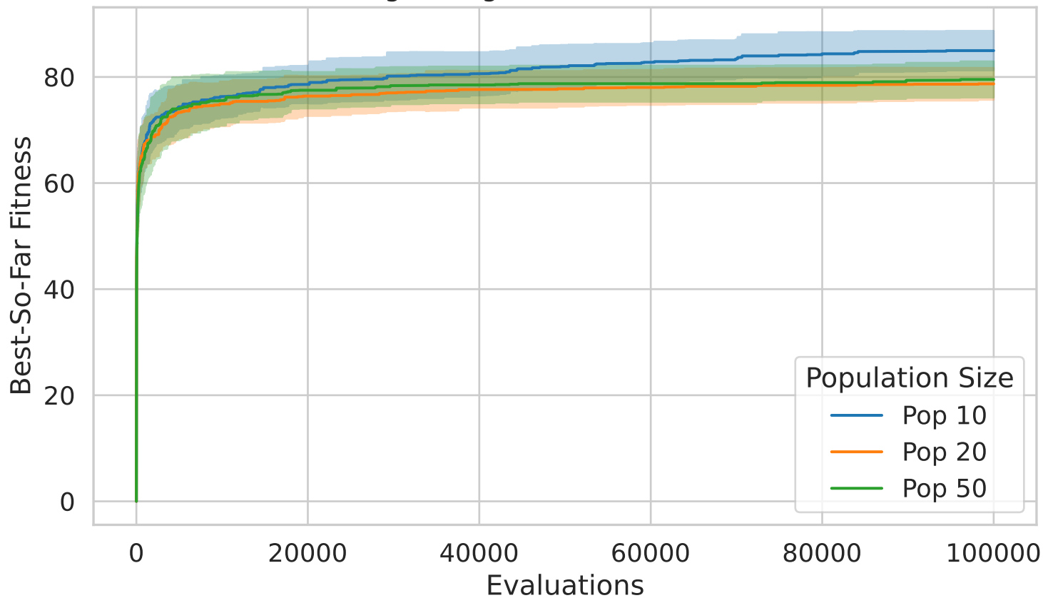
Fixed-Budget Progress – Instance 2202 (multi)
