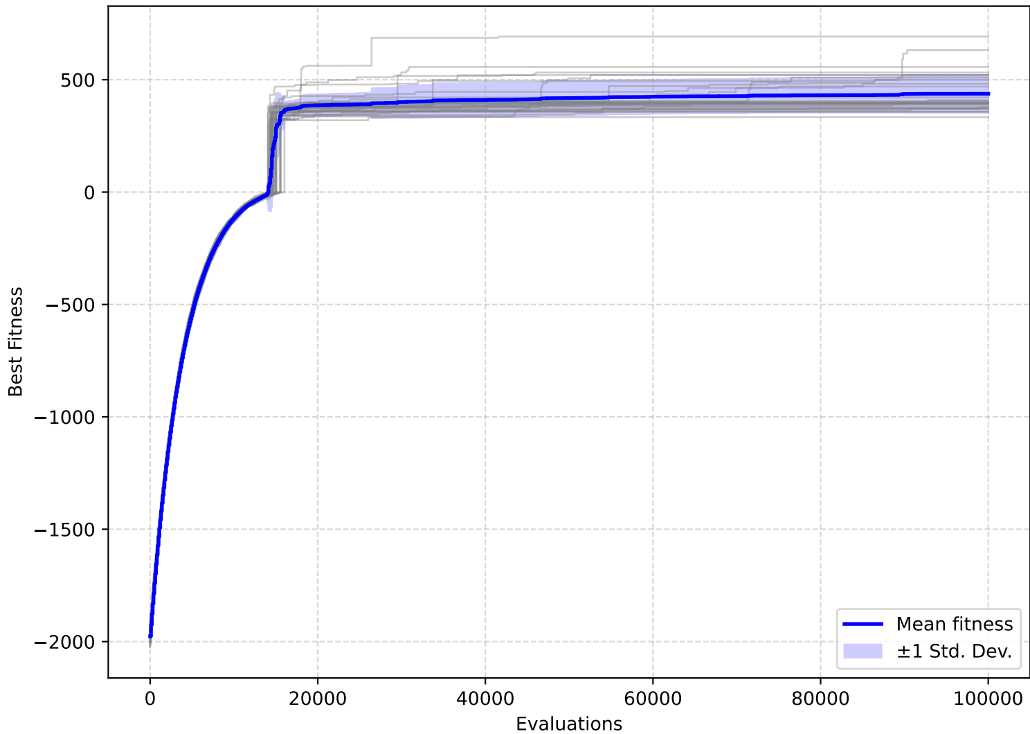
RLS/MaxInfluence — Convergence on F2202
