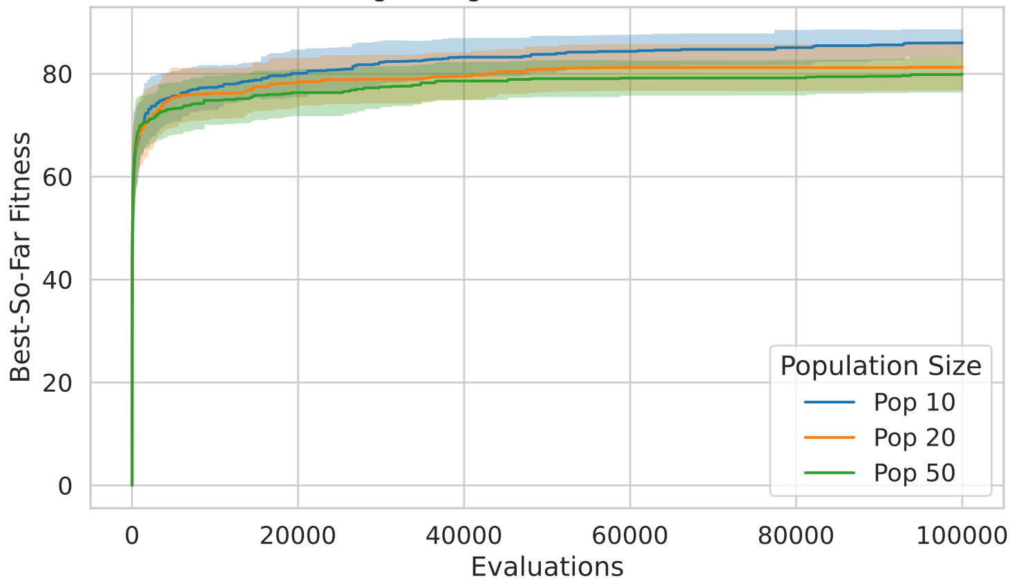
Fixed-Budget Progress – Instance 2201 (multi)
