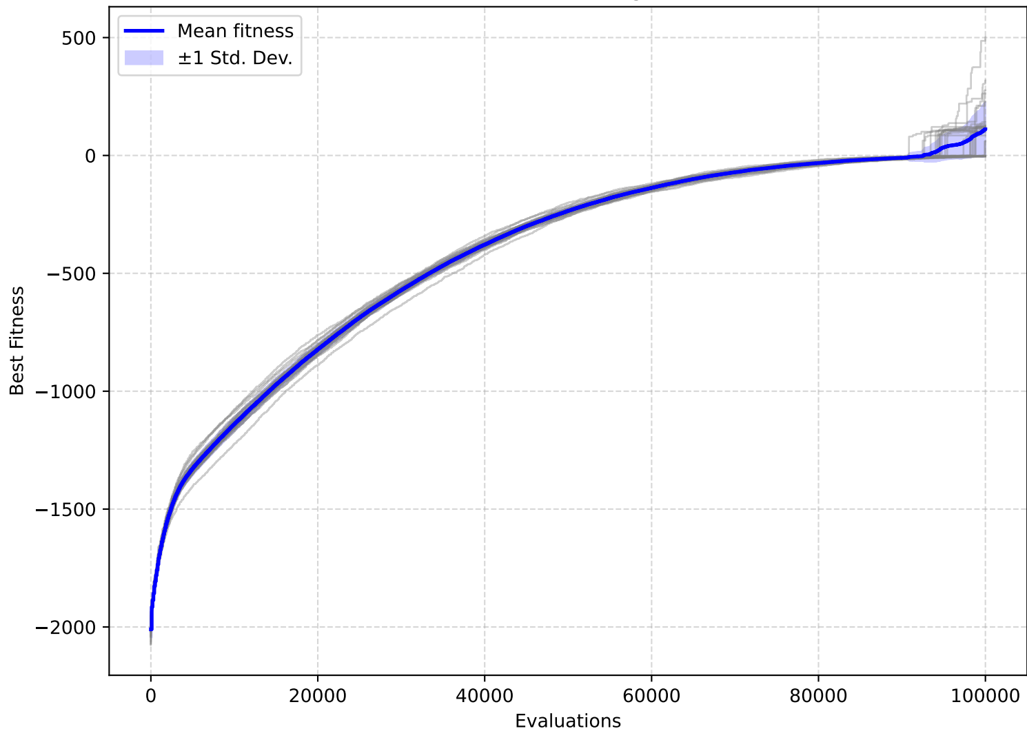
GA/MaxInfluence — Convergence on F2200
