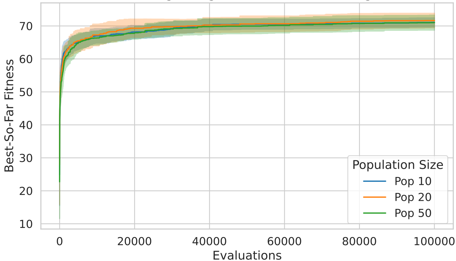
Fixed-Budget Progress - Instance 2201 (single)
