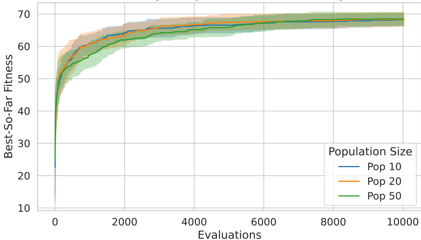
Fixed-Budget Progress - Instance 2200 (single)
