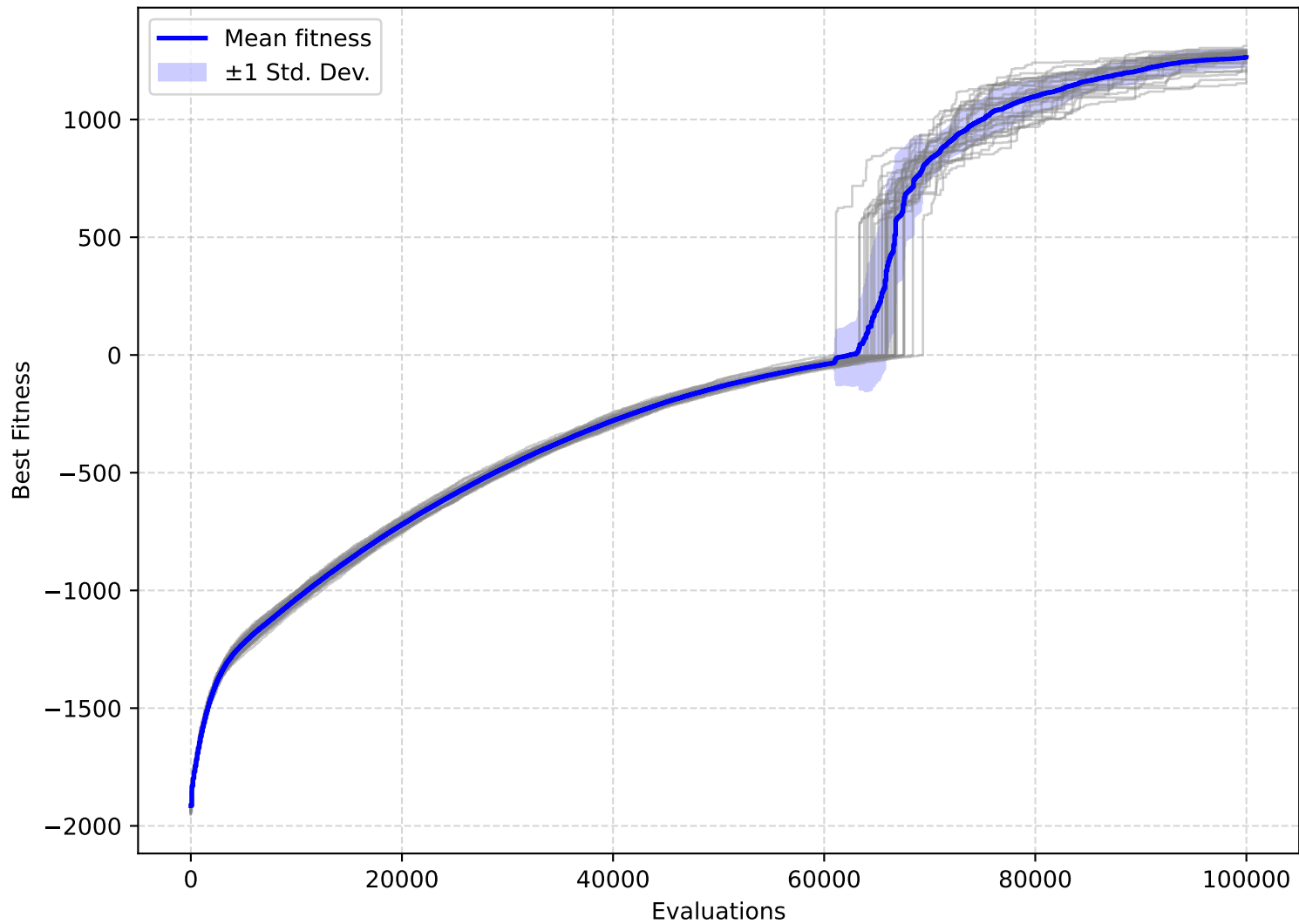
GA/MaxInfluence — Convergence on F2203
