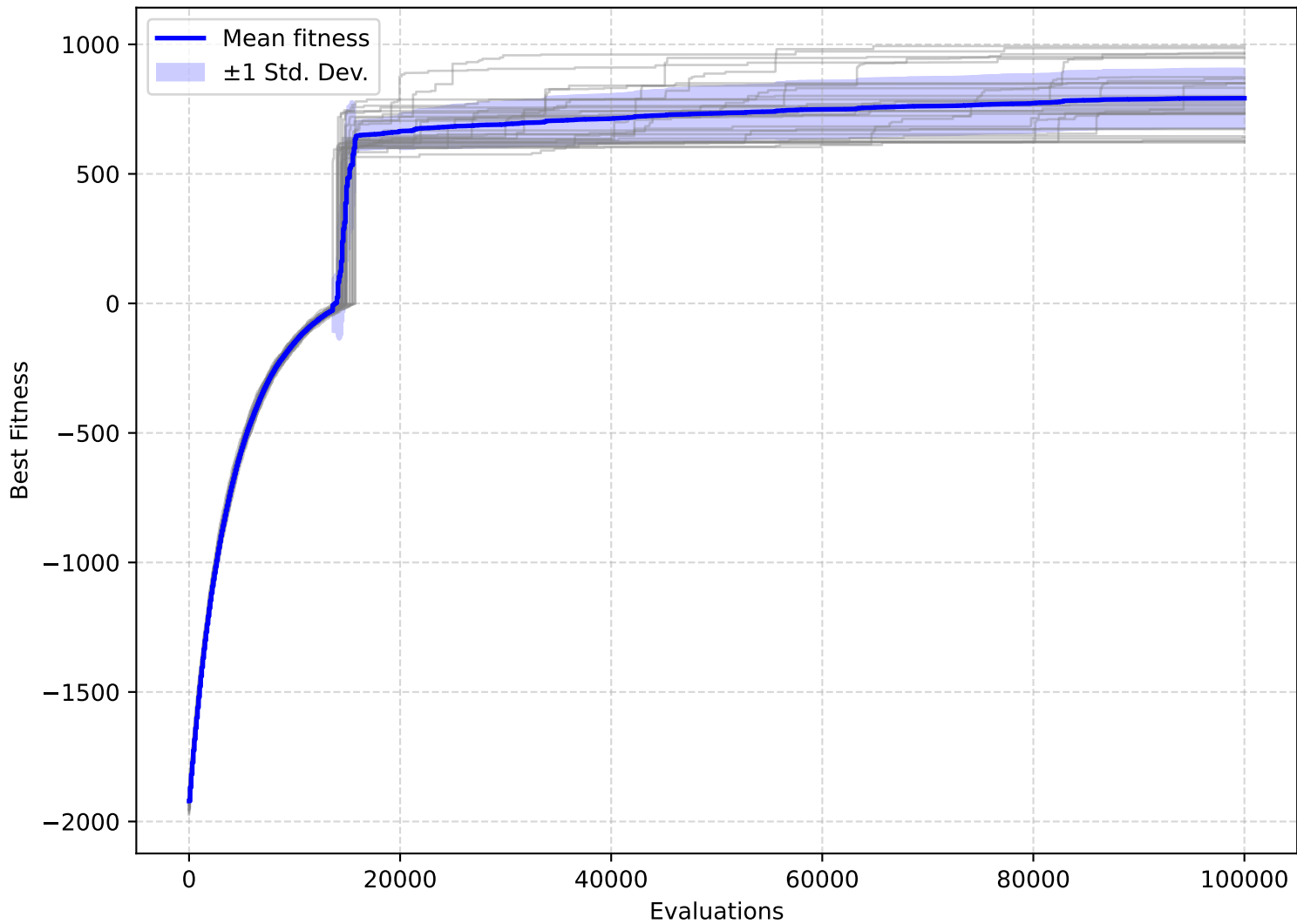
(1+1)EA/MaxInfluence — Convergence on F2203
