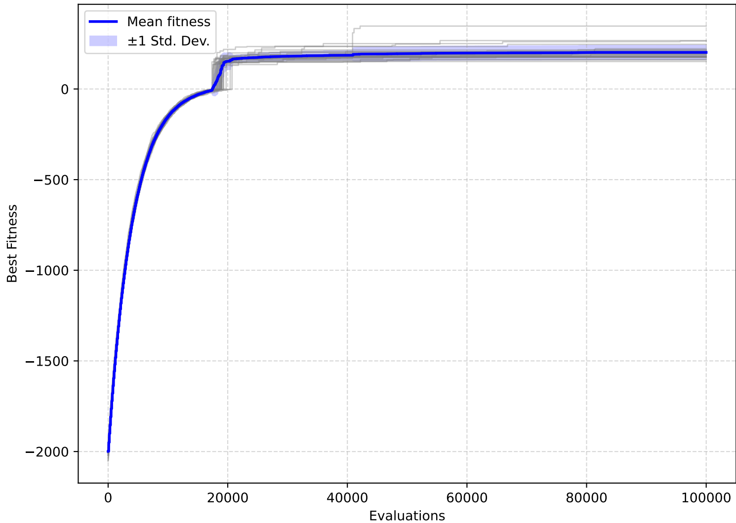
RLS/MaxInfluence — Convergence on F2201
