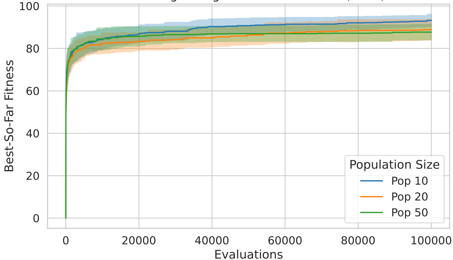
Fixed-Budget Progress - Instance 2102 (multi)
