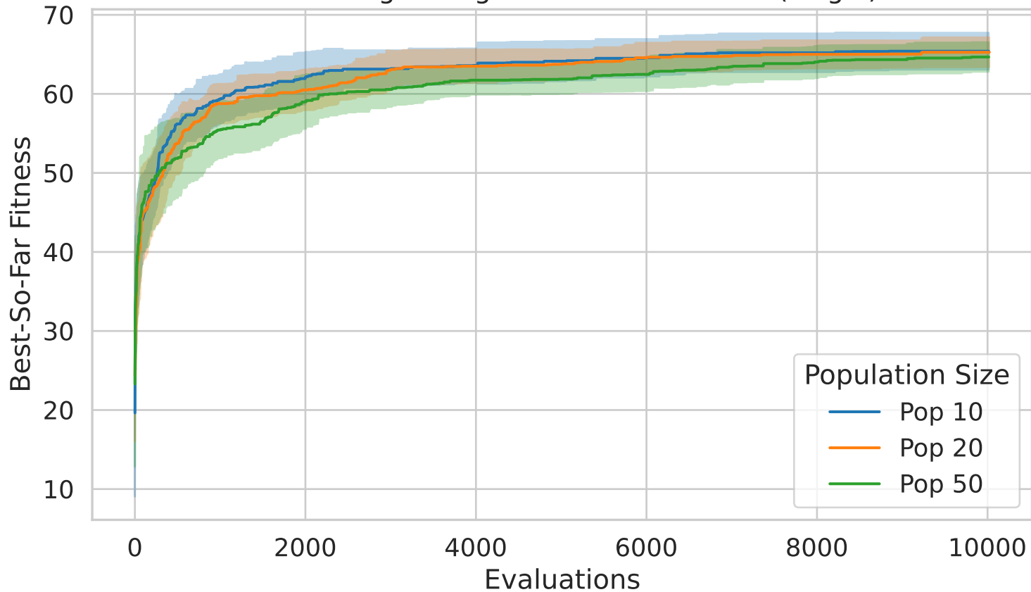
Fixed-Budget Progress - Instance 2101 (single)
