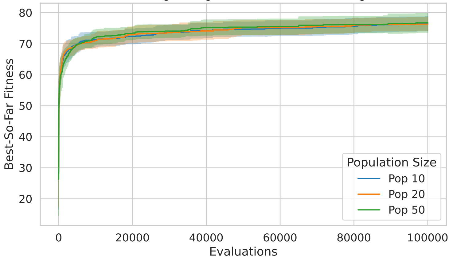
Fixed-Budget Progress – Instance 2102 (single)
