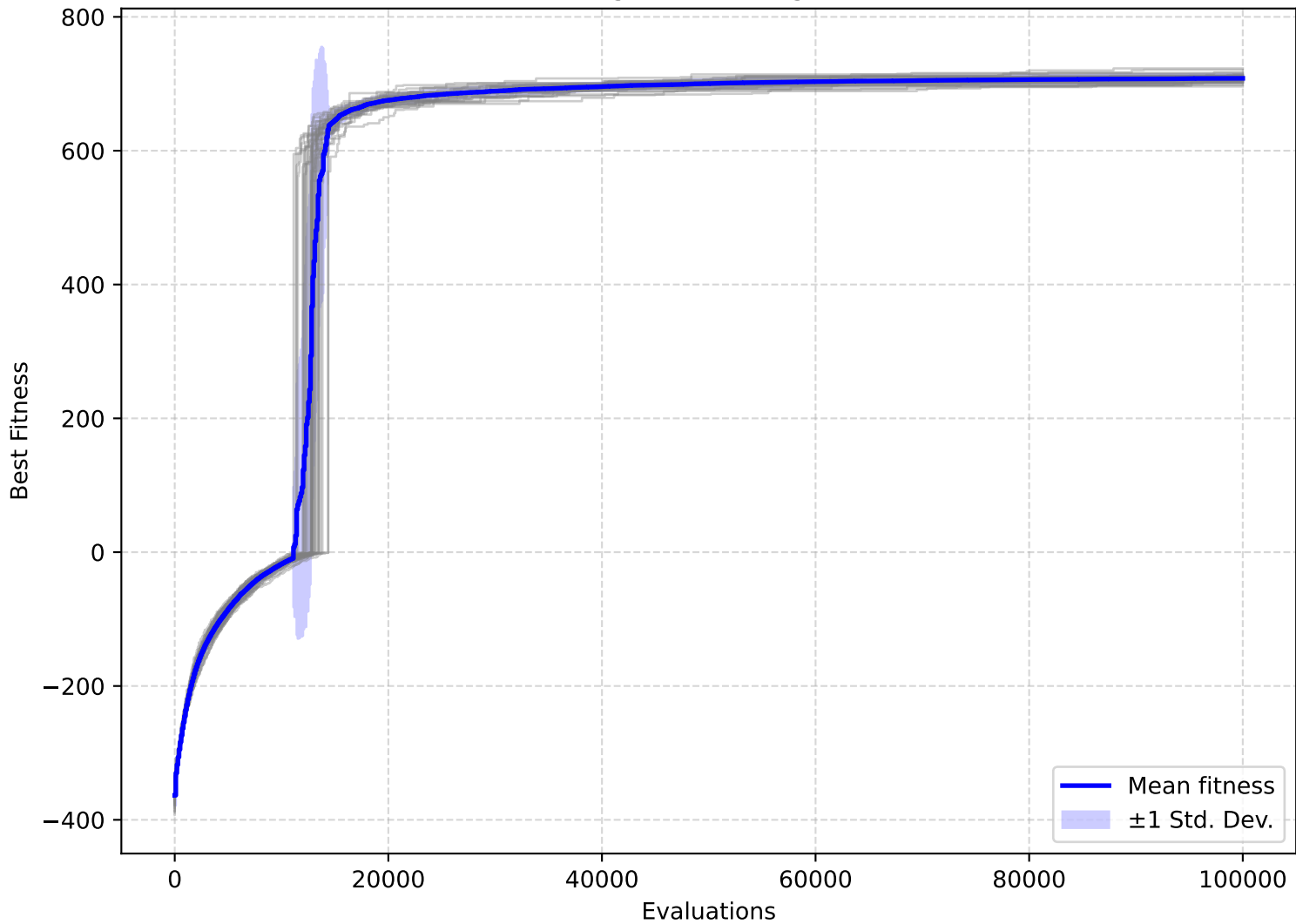
GA/MaxCoverage — Convergence on F2103
