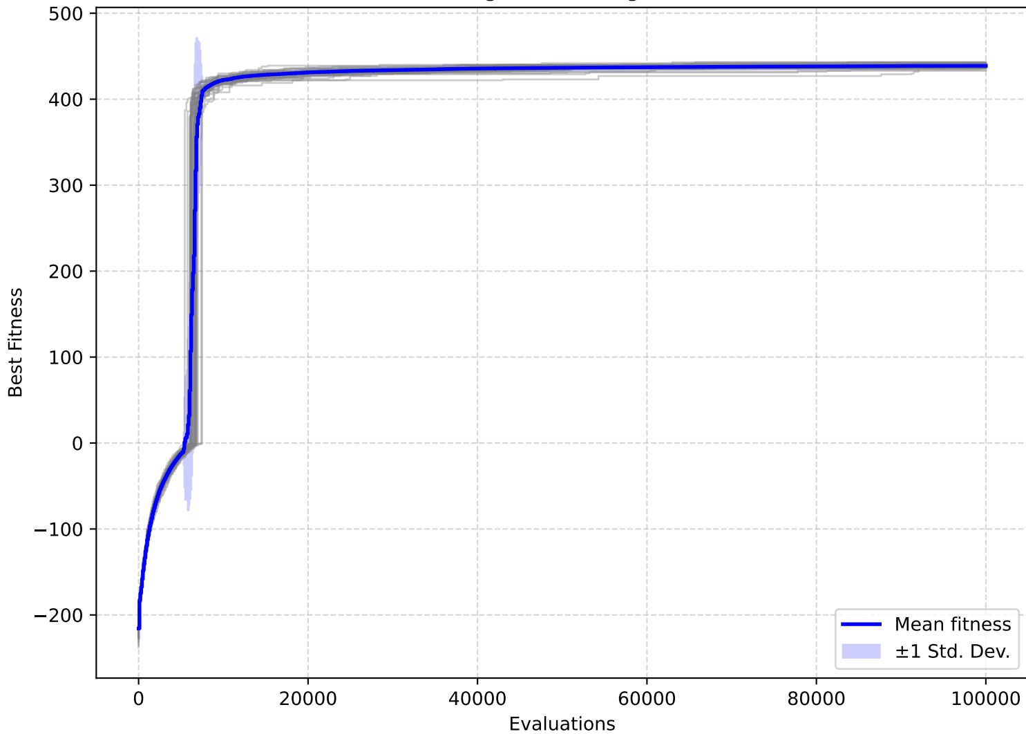
GA/MaxCoverage — Convergence on F2100
