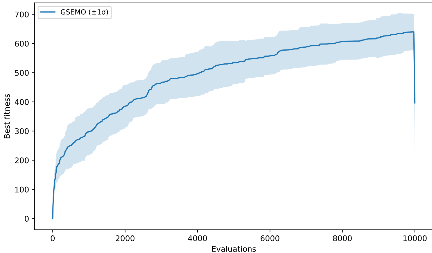
Fixed-Budget — Instance 2201
