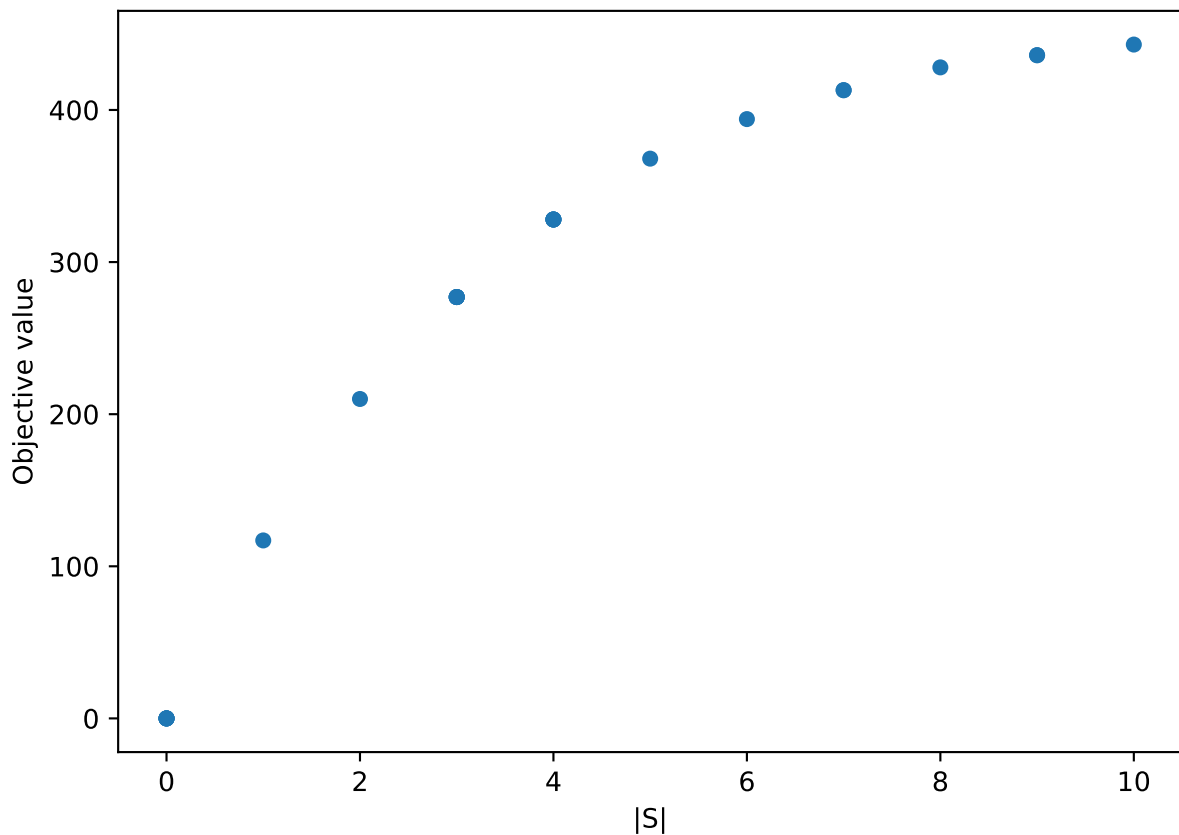
Trade-off - GSEMO - 2101
