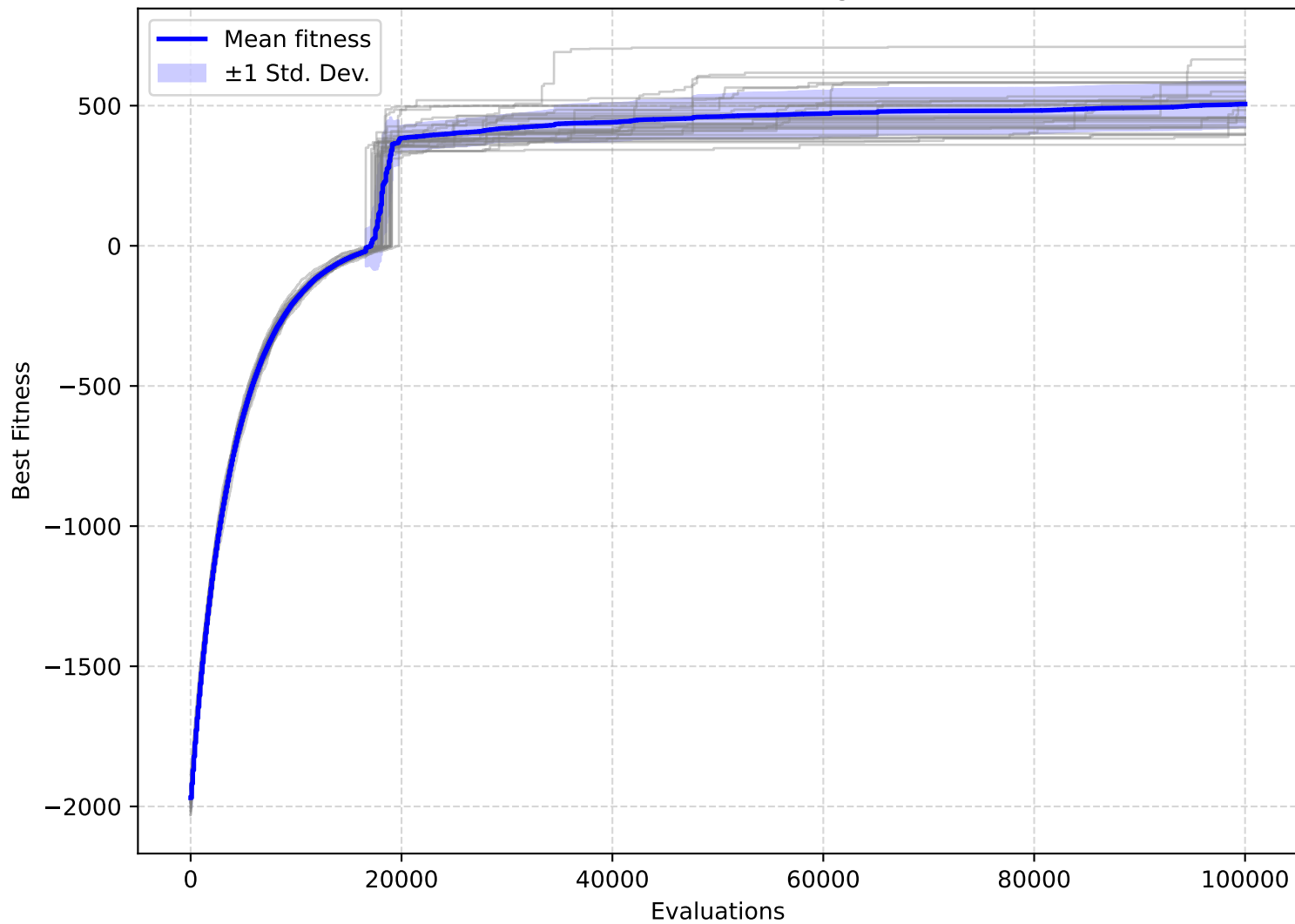
(1+1)EA/MaxInfluence — Convergence on F2202
