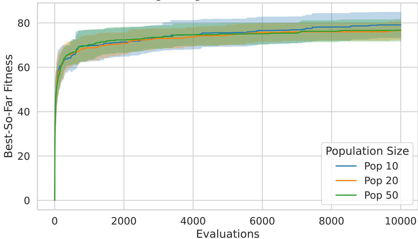
Fixed-Budget Progress – Instance 2200 (multi)
