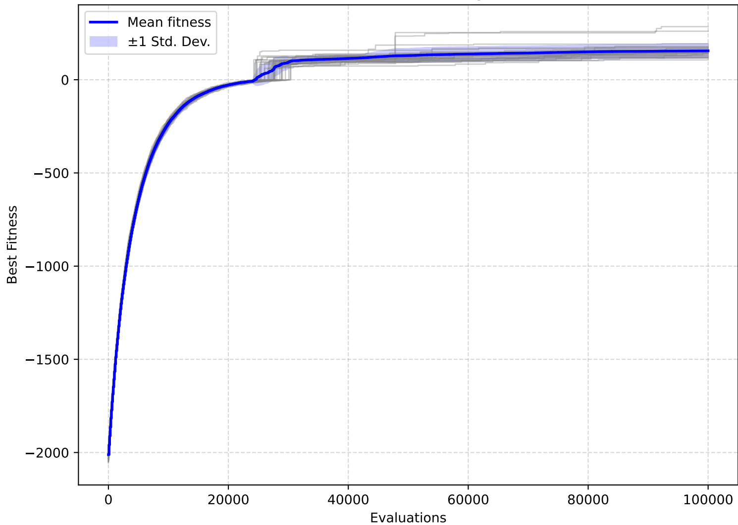
(1+1)EA/MaxInfluence — Convergence on F2200
