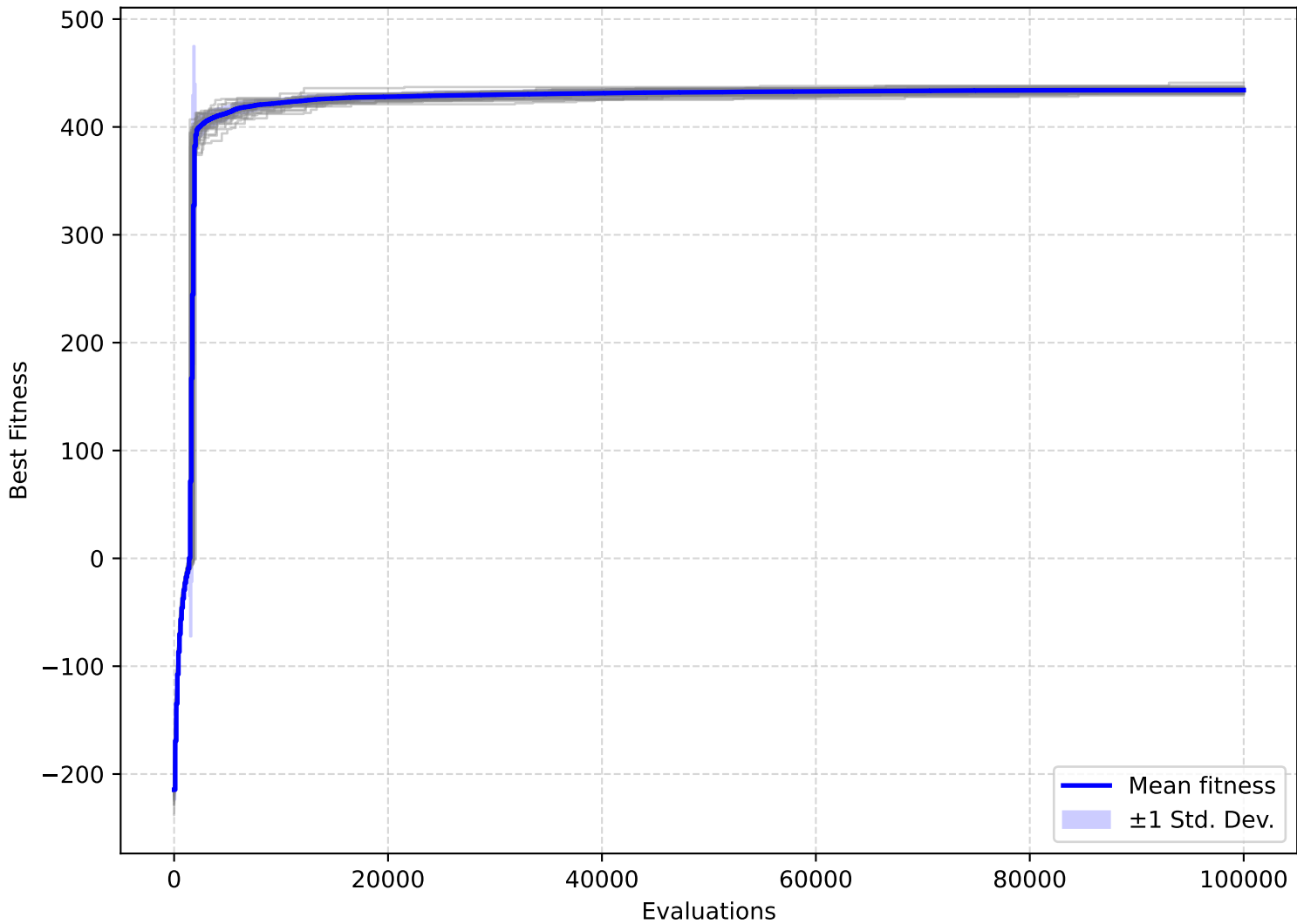
(1+1)EA/MaxCoverage — Convergence on F2100
