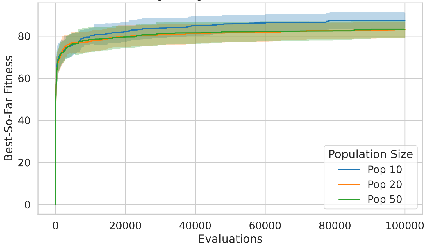
Fixed-Budget Progress – Instance 2203 (multi)
