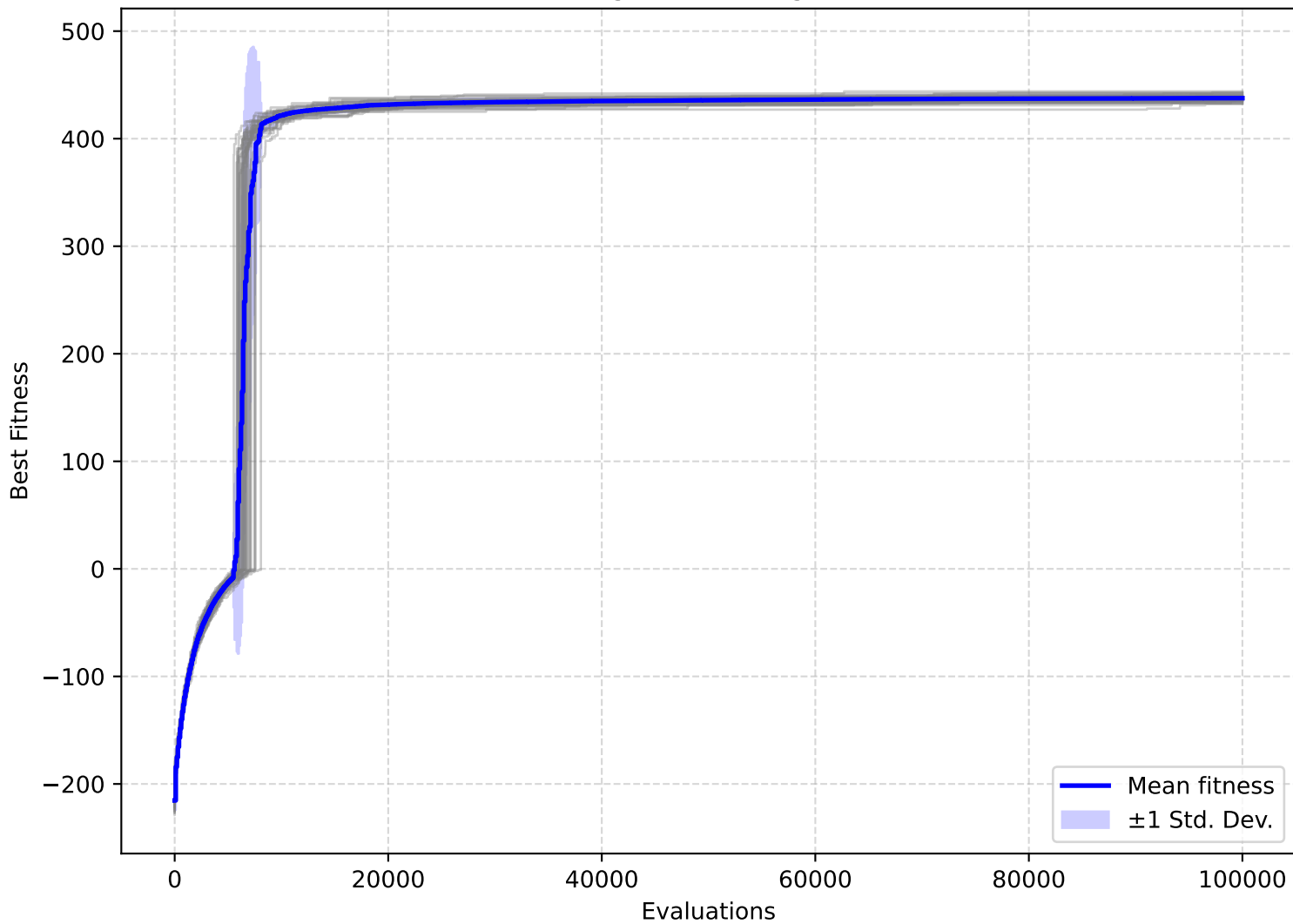
GA/MaxCoverage — Convergence on F2101
