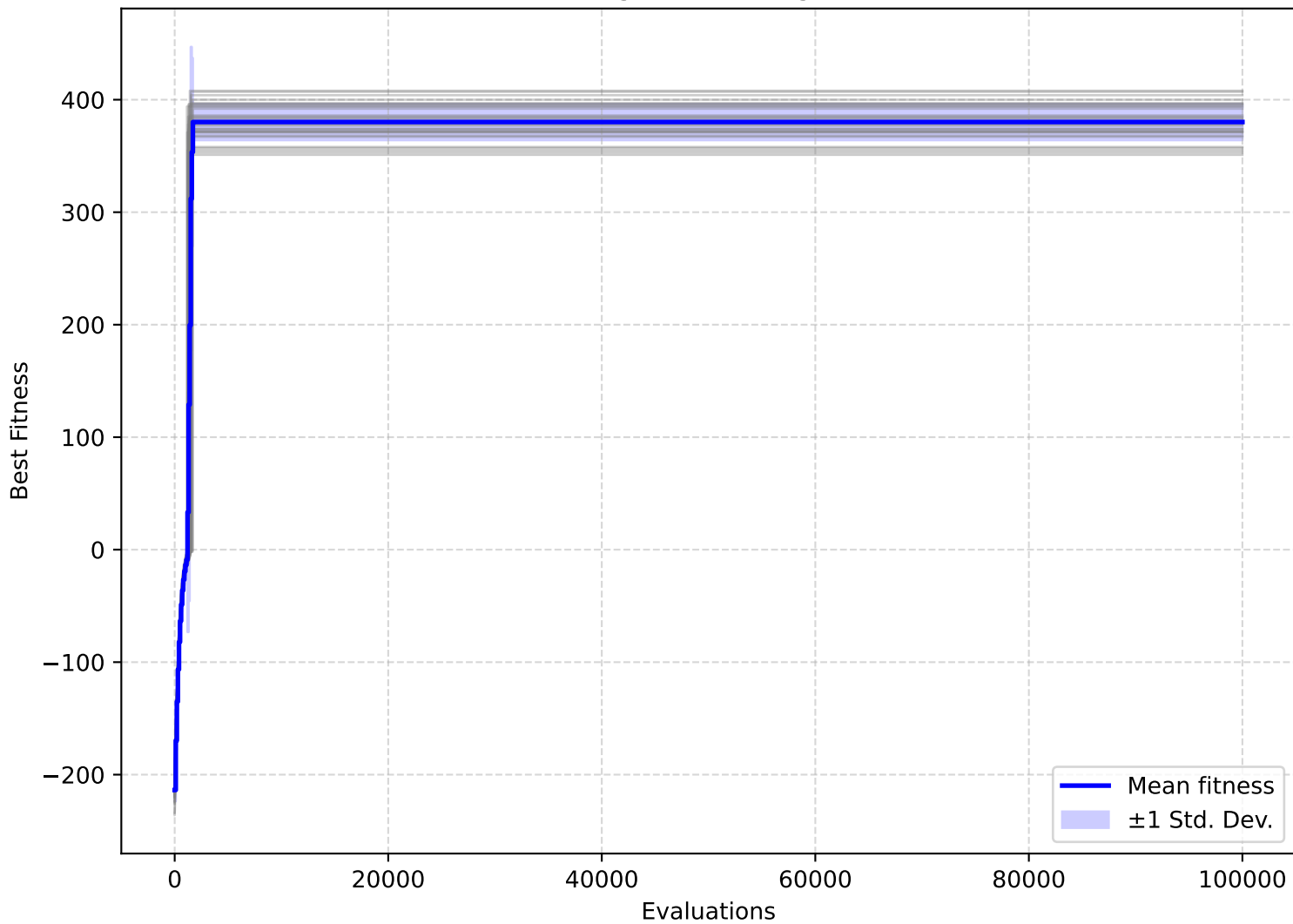
RLS/MaxCoverage — Convergence on F2100
