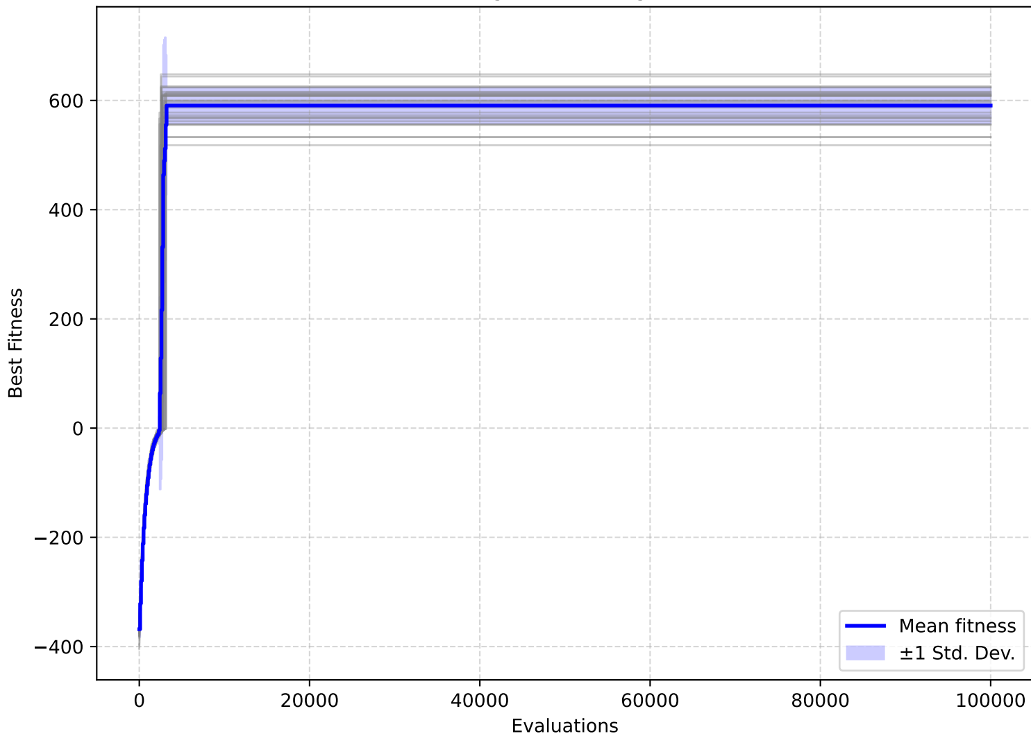
RLS/MaxCoverage — Convergence on F2103
