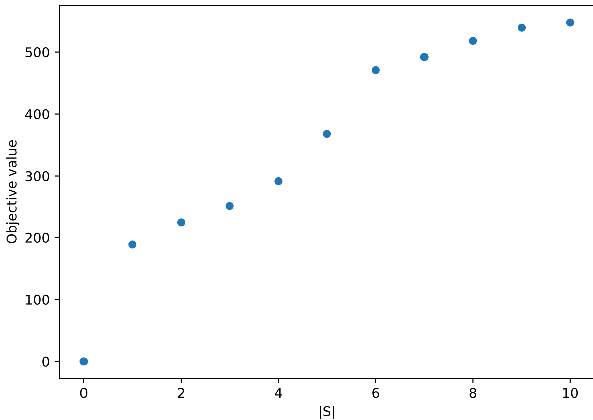
Trade-off - GSEMO - 2200
