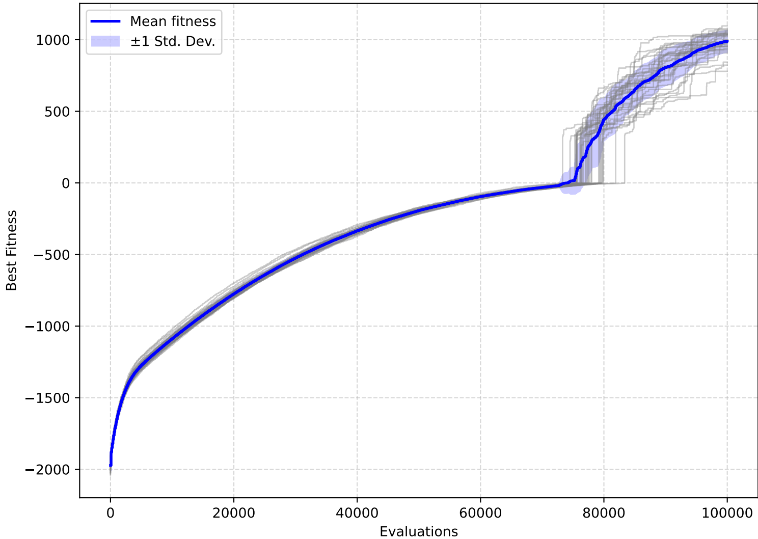
GA/MaxInfluence — Convergence on F2202
