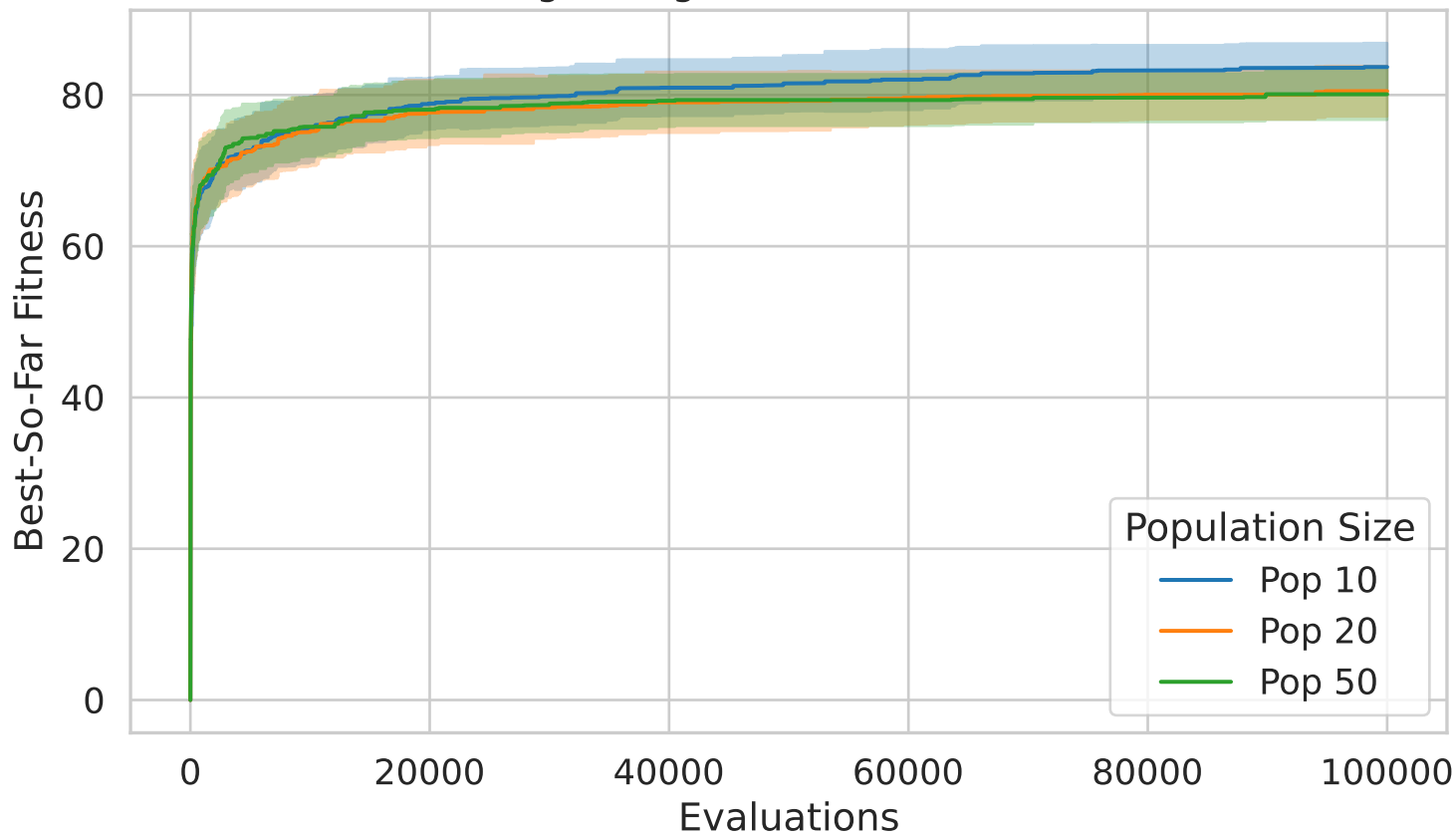
Fixed-Budget Progress – Instance 2103 (multi)
