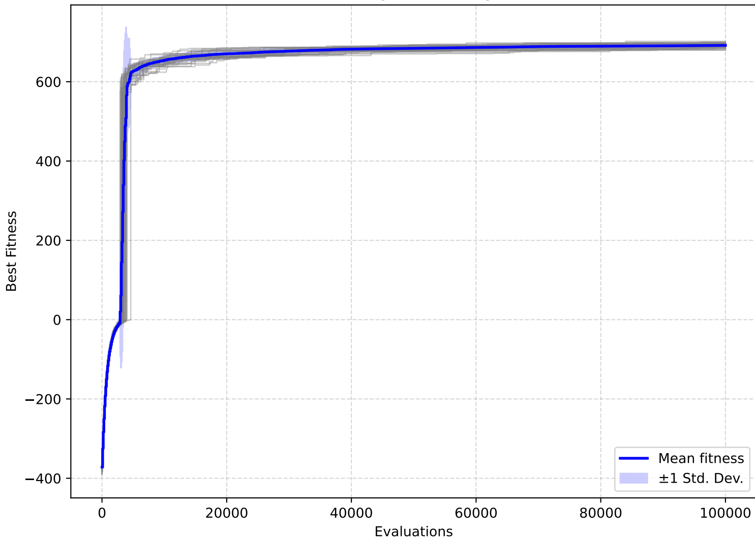
(1+1)EA/MaxCoverage — Convergence on F2103
