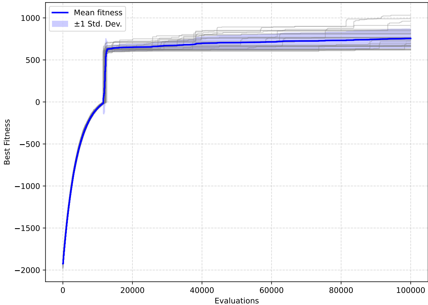
RLS/MaxInfluence — Convergence on F2203
