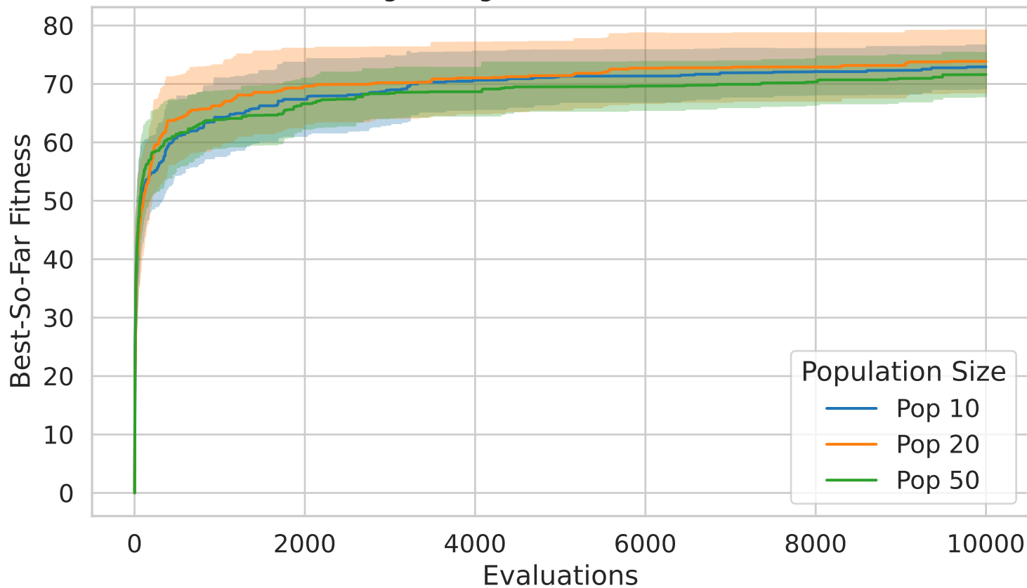
Fixed-Budget Progress – Instance 2101 (multi)
