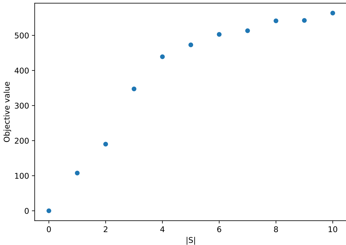
Trade-off - GSEMO - 2202
