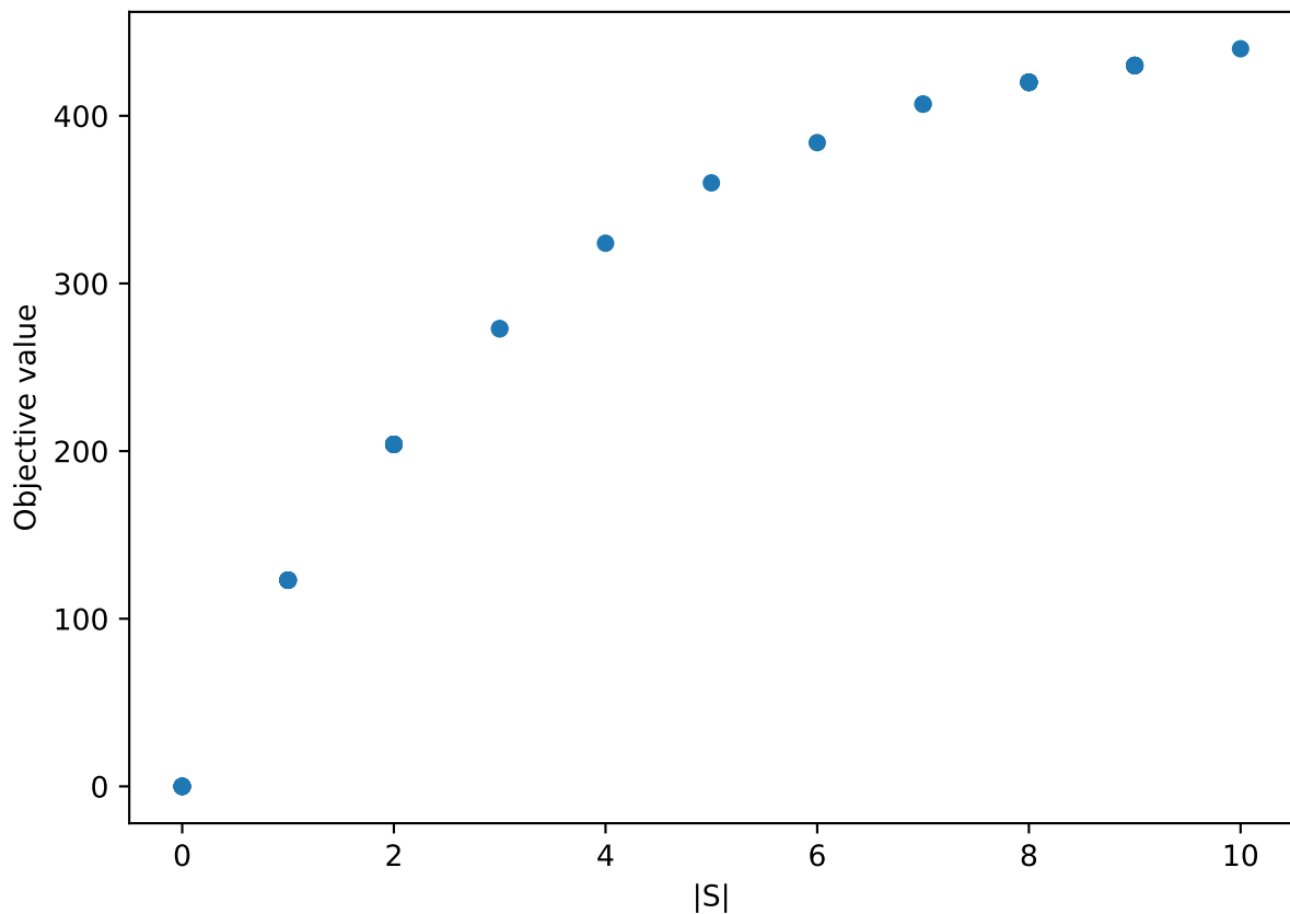
Trade-off - GSEMO - 2100
