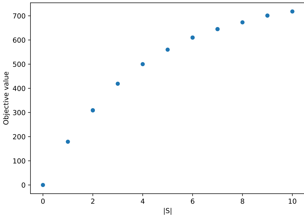
Trade-off - GSEMO - 2103
