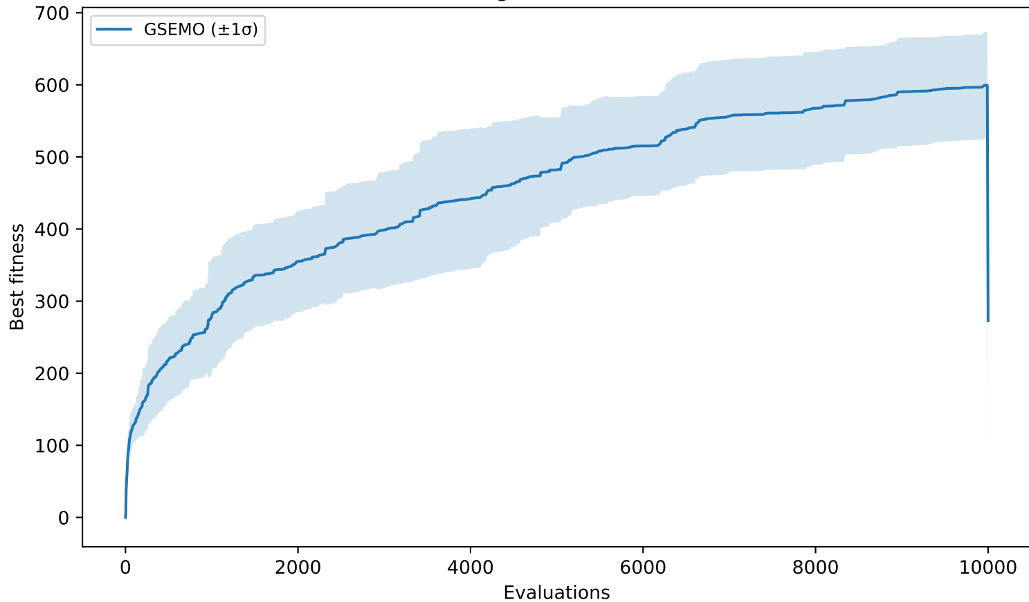
Fixed-Budget — Instance 2200
