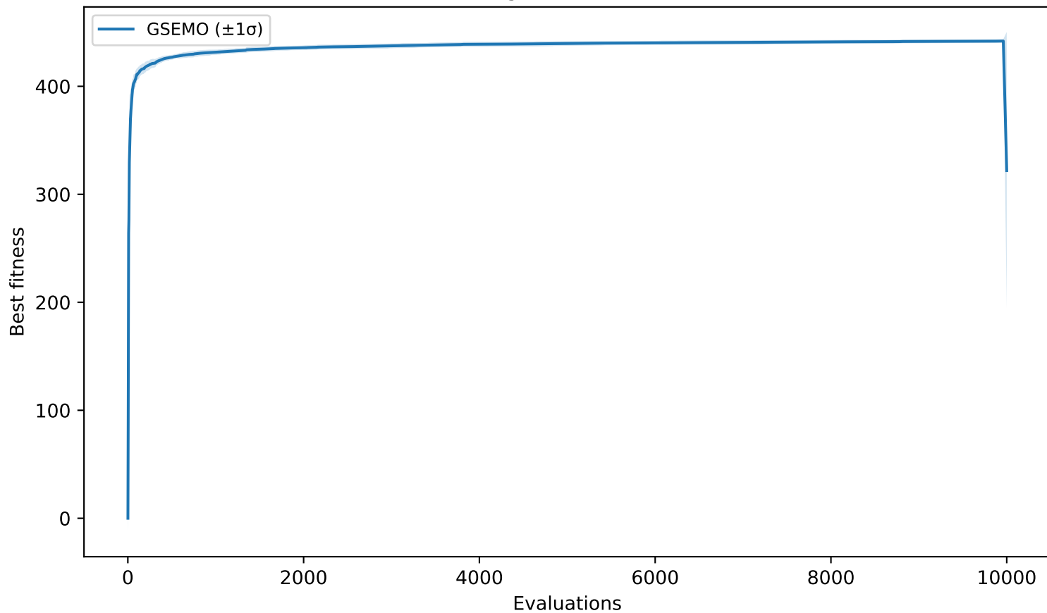
Fixed-Budget — Instance 2101
