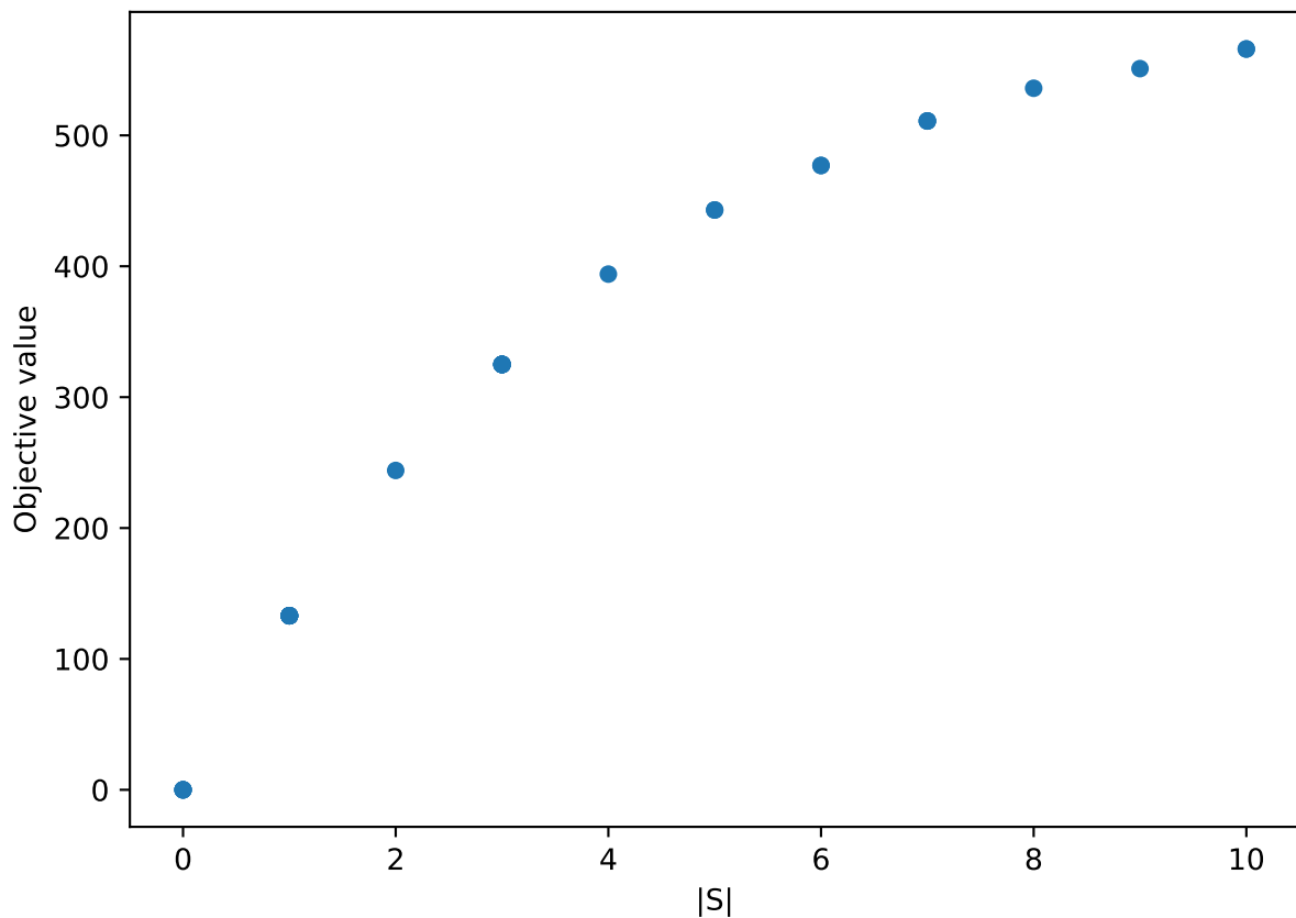
Trade-off - GSEMO - 2102
