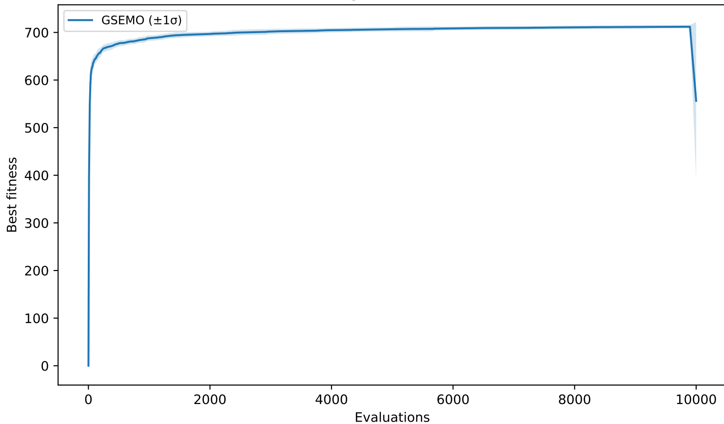
Fixed-Budget — Instance 2103
