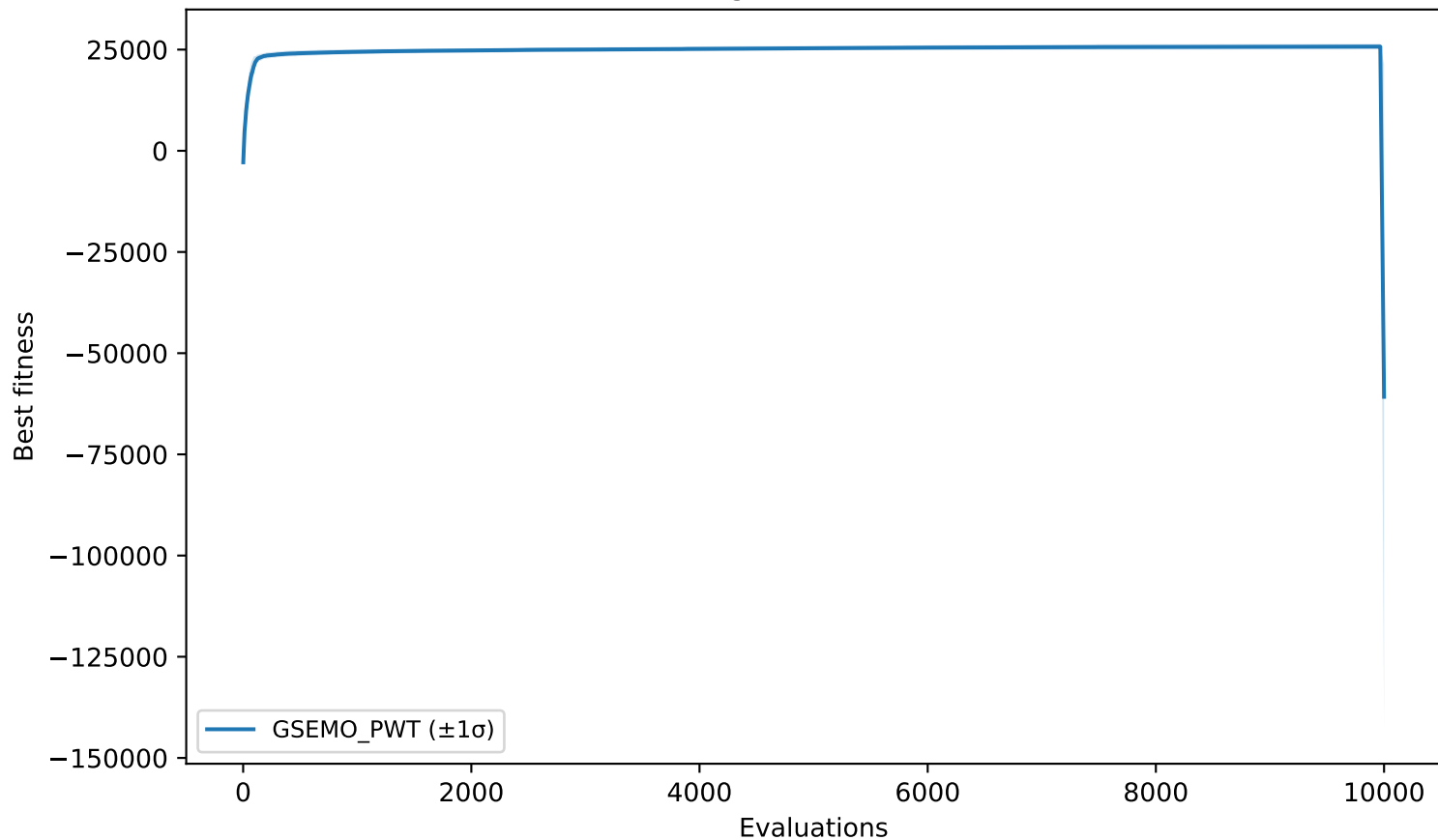
Fixed-Budget — Instance 2300
