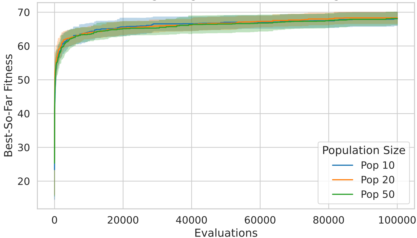
Fixed-Budget Progress - Instance 2202 (single)
