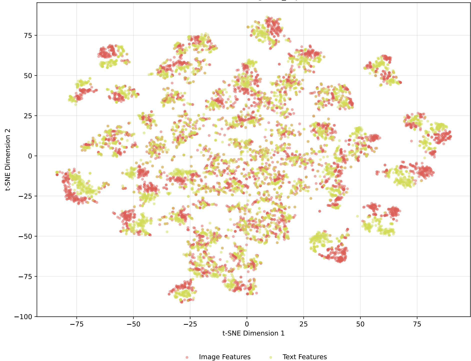
t-SNE Visualization of ImageNet_caption Features
