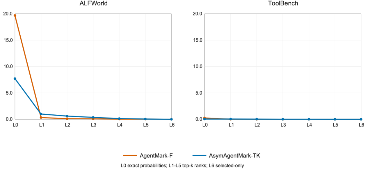
Figure 4. Effective capacity over the L0–L6 verifier-channel ladder. AgentMark-F has high exact-channel capacity on ALFWorld but loses usable capacity as soon as the verifier only has ranks. AsymAgentMark-TK gives up some exact-channel capacity but degrades more gradually under top- k rank views.
