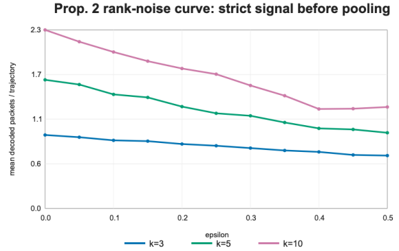
Figure 5. Fine-grid ToolBench rank-noise diagnostic before pooling. Pooled recovery stays near saturation, but the per-trajectory packet budget decreases with adjacent-swap noise; larger k exposes more packets and also loses more absolute packet budget as \epsilon grows.
