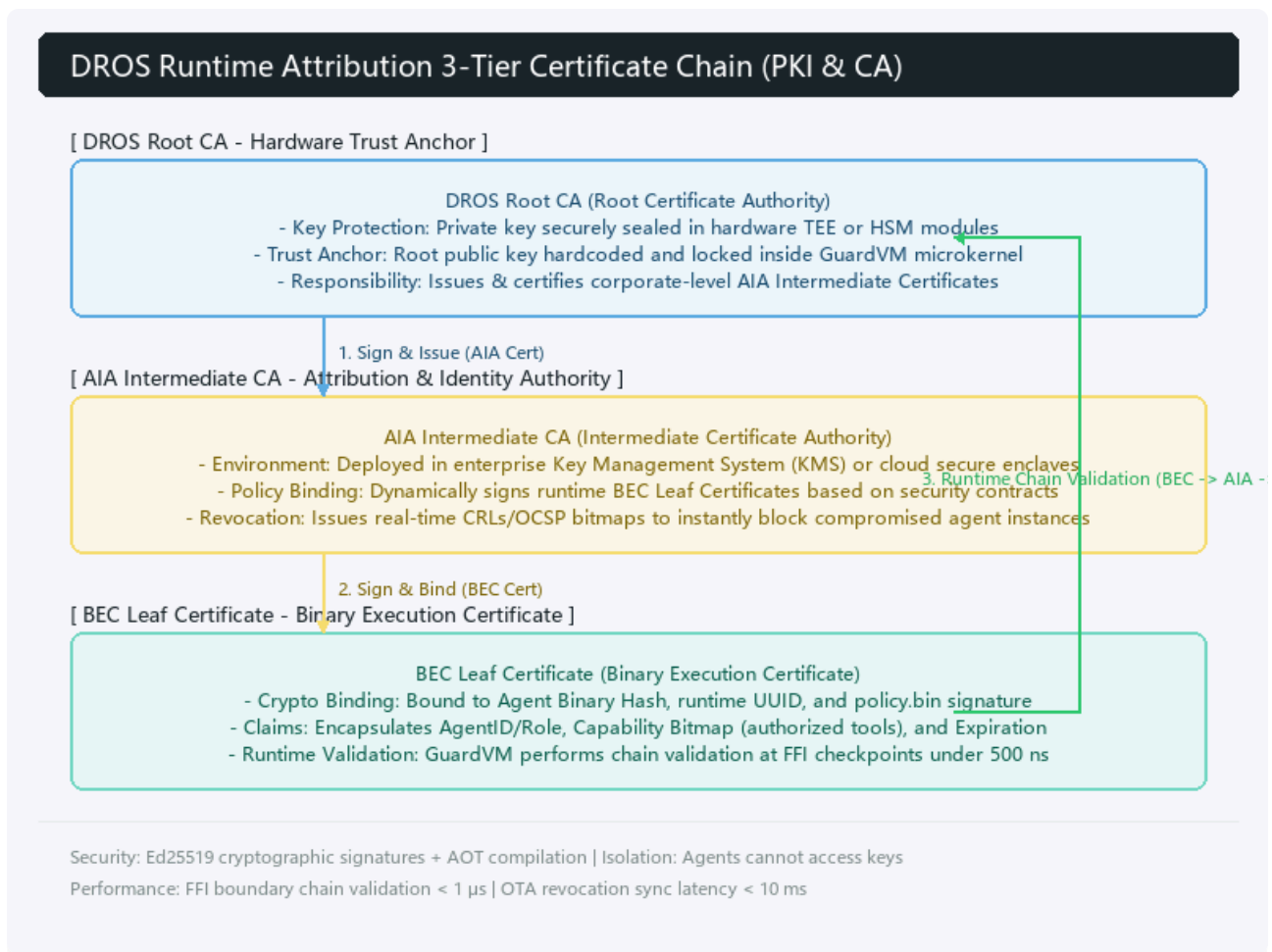
Figure 2: DROS Agent Three-Tier Certificate Chain Key Management
