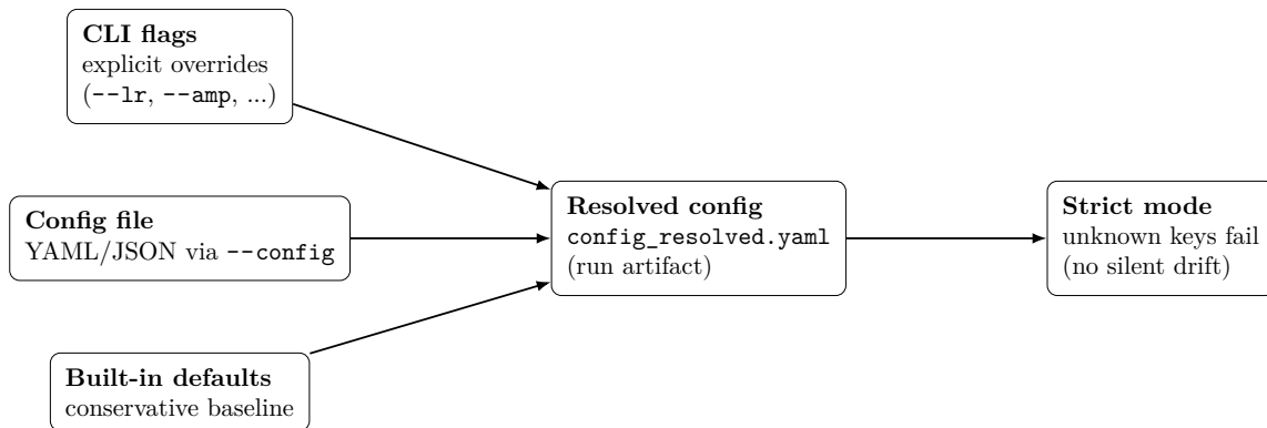
Figure 12.2: Configuration resolution: the run contract enforces explicit keys and produces a resolved config artifact.
