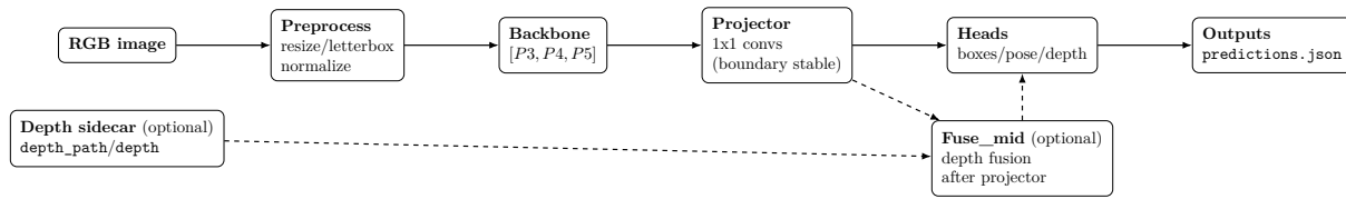
Figure 10.2: Depth modes: sidecar carries depth as metadata; fuse_mid fuses depth after the projector (outside the backbone swap boundary).
