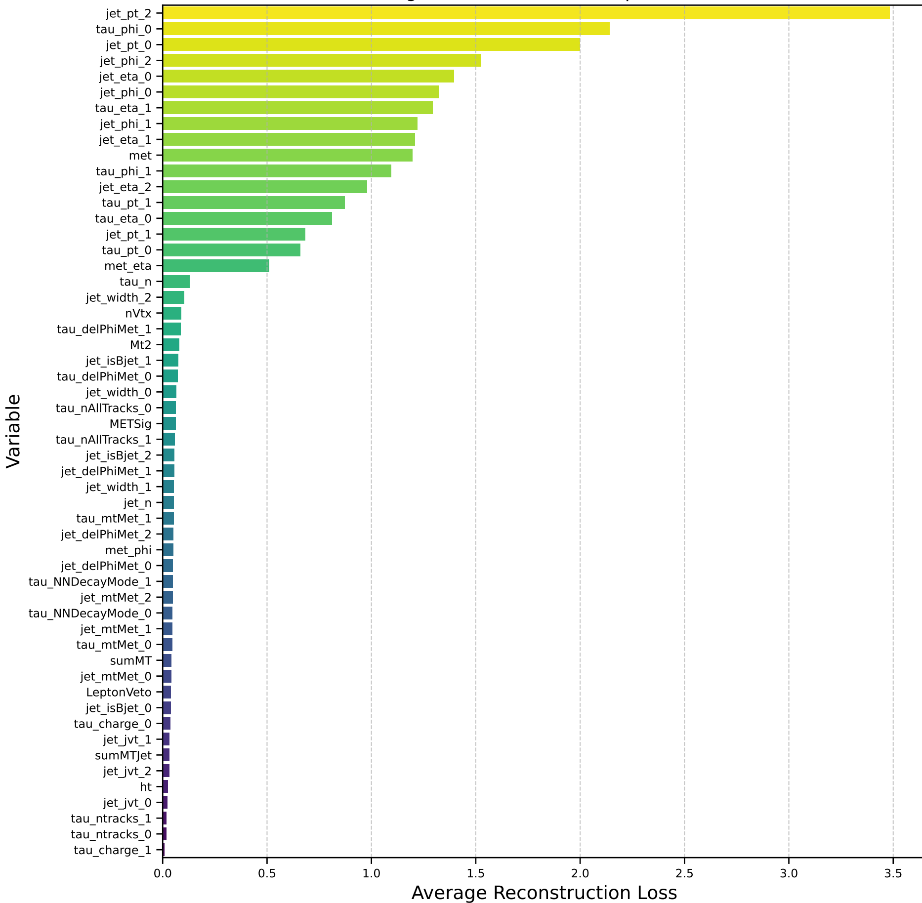
Average Reconstruction Loss per Variable
