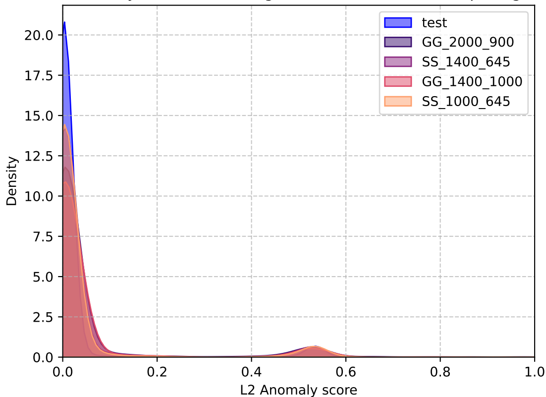
L2 Anomaly Scores for background test-set and example signals
