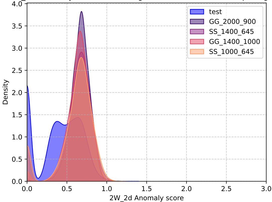
2W_2d Anomaly Scores for background test-set and example signals
