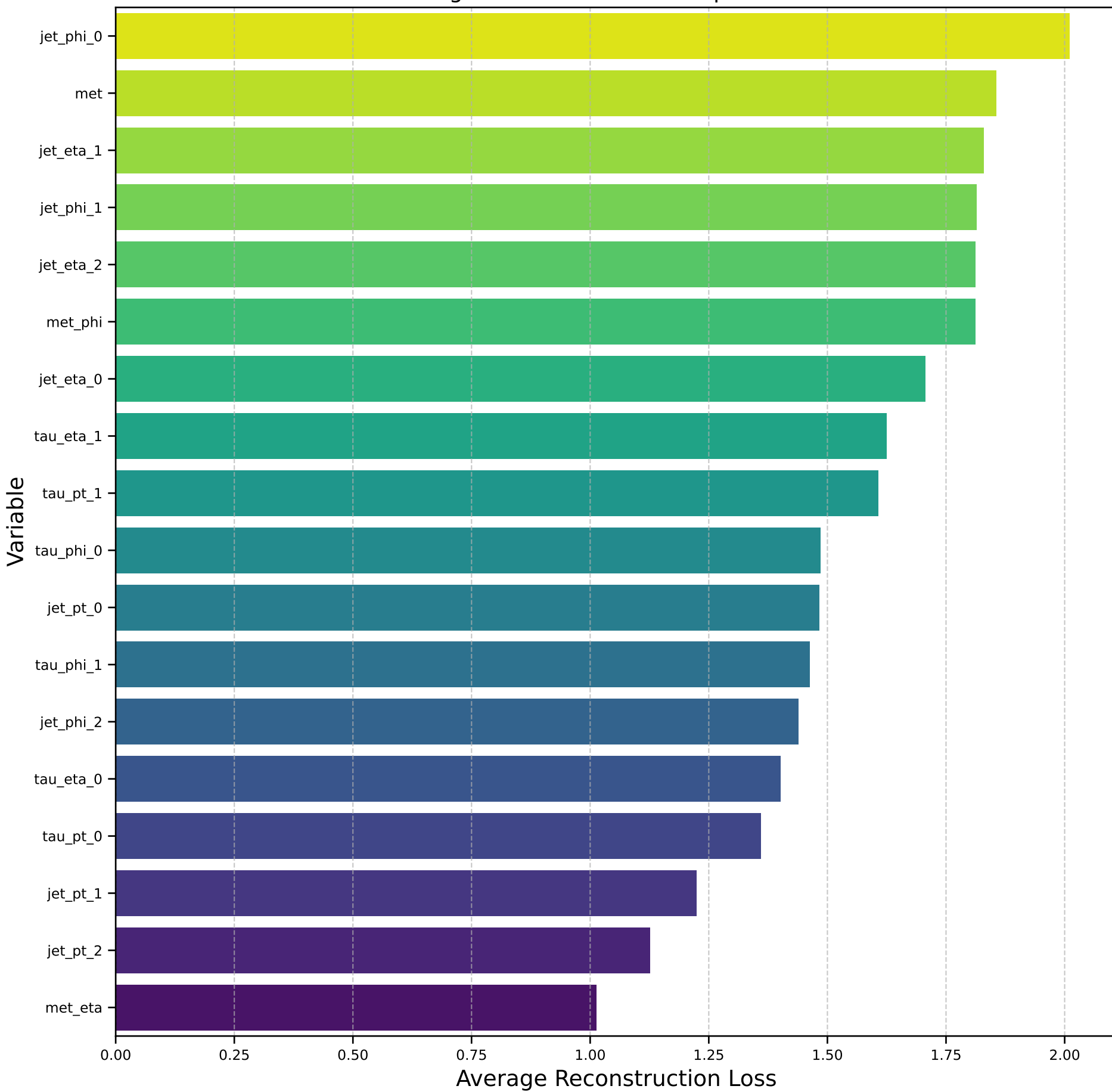
Average Reconstruction Loss per Variable
