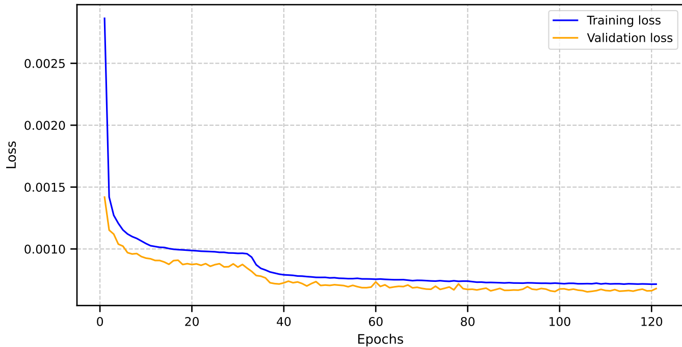
Loss comparison
