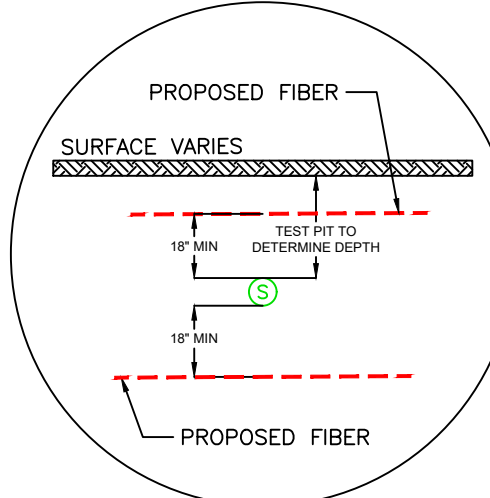
SEWER DETAIL SCALE: NTS
