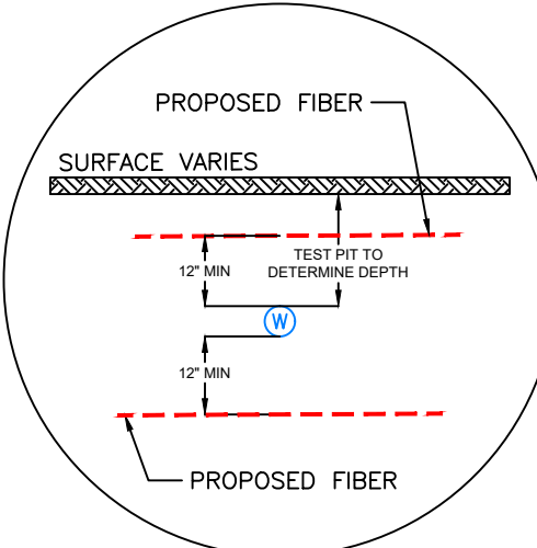
WATER DETAIL SCALE:NTS
