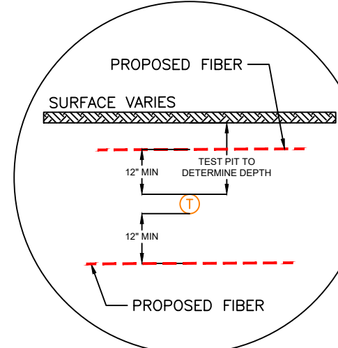
TELEPHONE DETAIL SCALE:NTS
