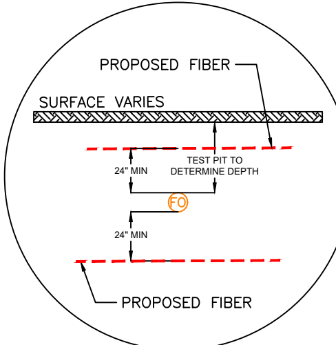
FIBER DETAIL SCALE:NTS
