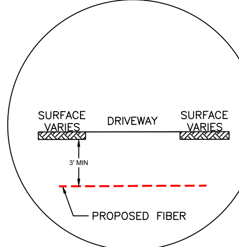
DRIVEWAY/PRIVATE RD SCALE:NTS
