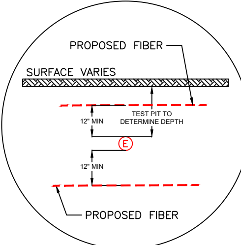
ELECTRIC DETAIL SCALE:NTS
