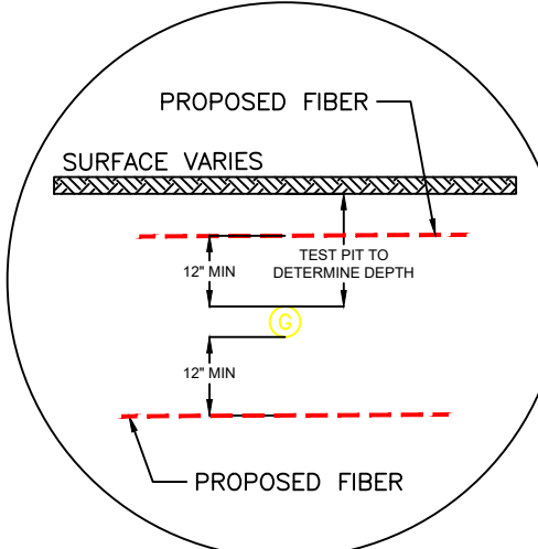
GAS DETAIL SCALE:NTS
