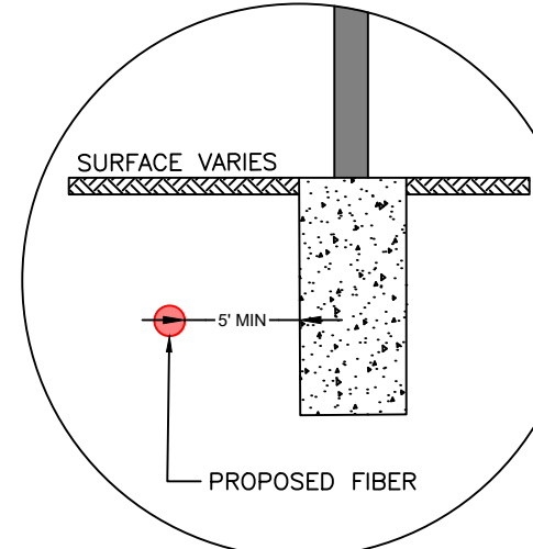
TRAFFIC SIGNAL DETAIL SCALE:NTS
