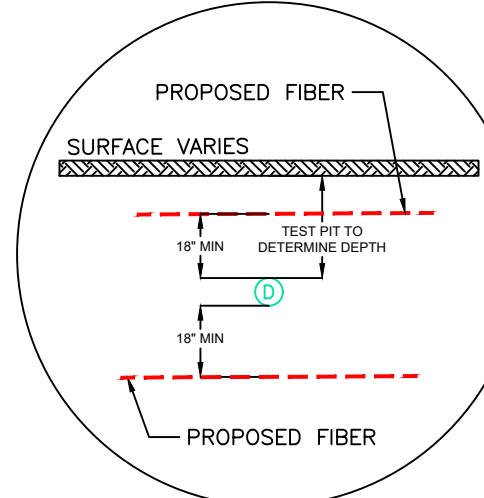
STORM DRAIN DETAIL SCALE:NTS
