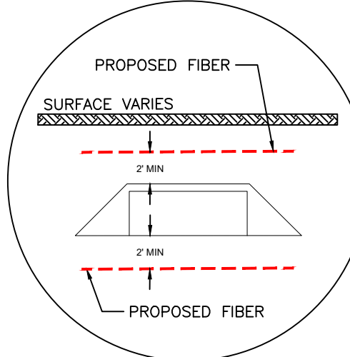
CULVERT DETAIL SCALE:NTS
