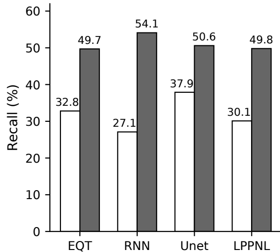
(a) Recall
