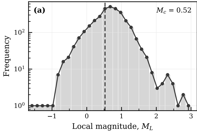
Non-cumulative FMD
