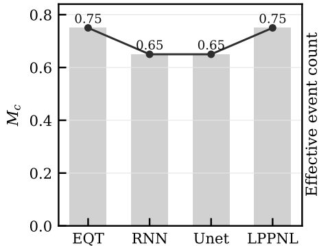
(b) MAXC M_c
