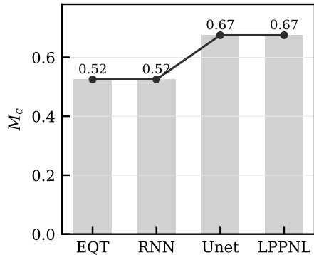
(a) Cumulative-fit M_c
