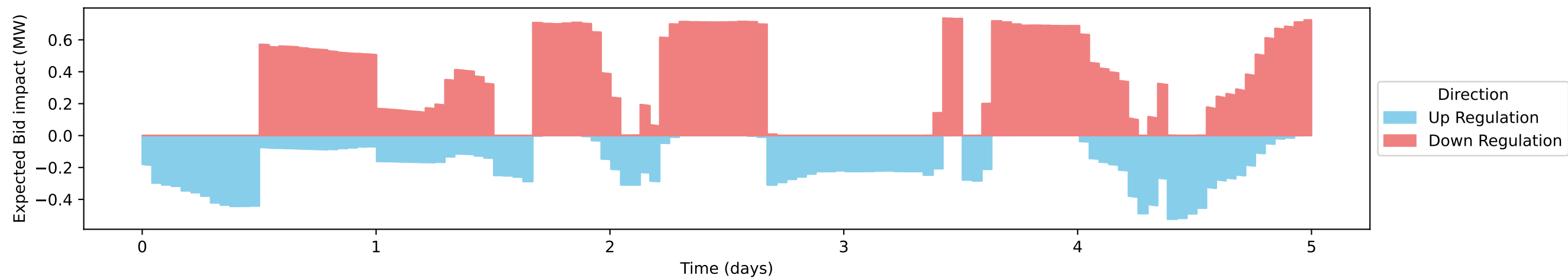
complete_MPC Expected consumption impact of bids (MW) (2024-10-10, SE1)
