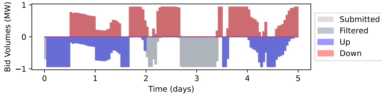
complete_MPC activated prices and volumes. (2024-10-10, SE1)
