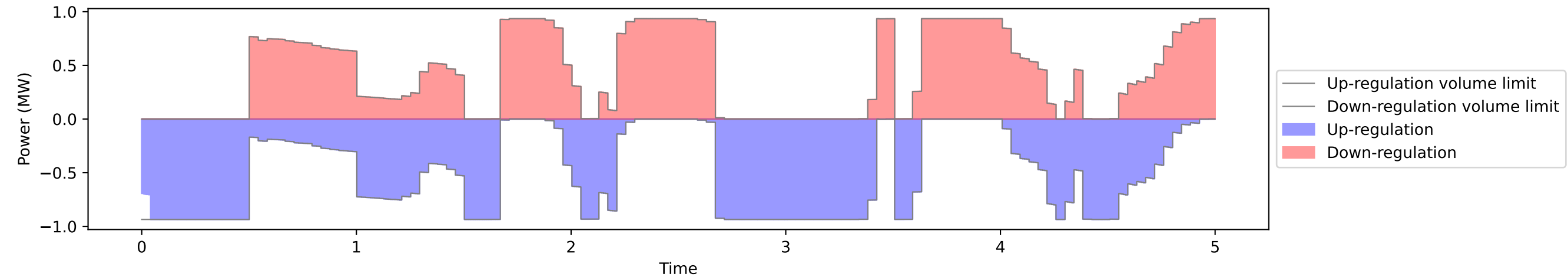
complete_MPC volumes in MW (2024-10-10, SE1)
