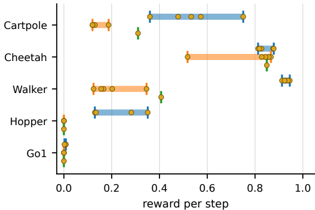
Environment reward
