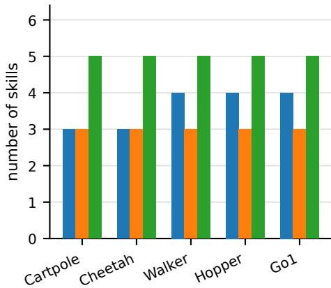
Skill count
