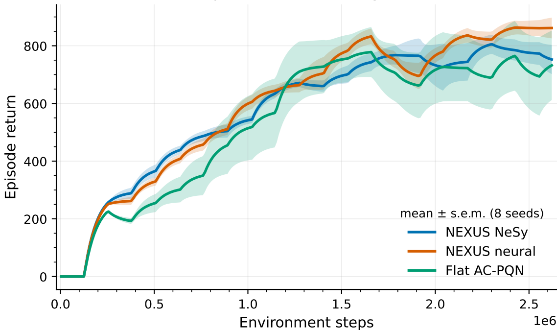
CartpoleBalance: training return
