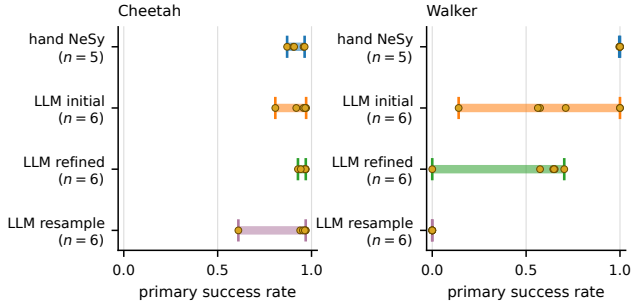
Fig. 11. Task success on Cheetah and Walker at a matched RL training budget. Hand-written NeSy is compared with initial, once-refined, and independently resampled specifications. All are trained from scratch. Cheetah is comparatively stable; Walker varies across proposals, and resampling performs poorly.
