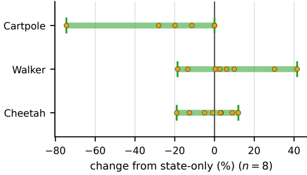
Fig. 12. Seed-matched percentage change in the evaluation score from state-only to state+camera on Cartpole, Walker, and Cheetah, computed as 100 \times (\text{camera} - \text{state-only}) / \text{state-only} . Each environment has n = 8 points: three 30-episode runs plus five 64-episode runs on Cartpole and Walker, and three 30-episode runs plus five changes recorded only as percentages on Cheetah. Positive values indicate improvement; negative values indicate a decrease. These relative changes should not be interpreted as a common task-success scale across environments.
