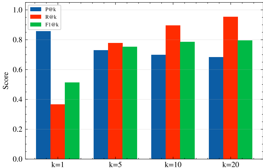
Precision/Recall/F1 at k
